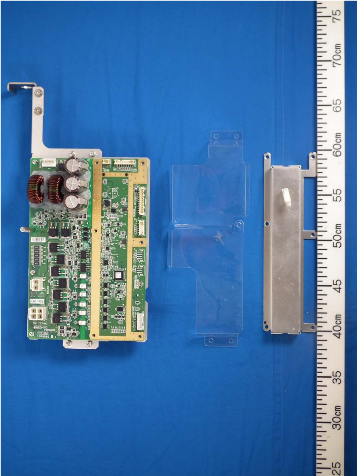
1.1.7 MTR-DRV module (with the shielding/plastic cover removed, showing MTR-DRV Board 03P9560)
