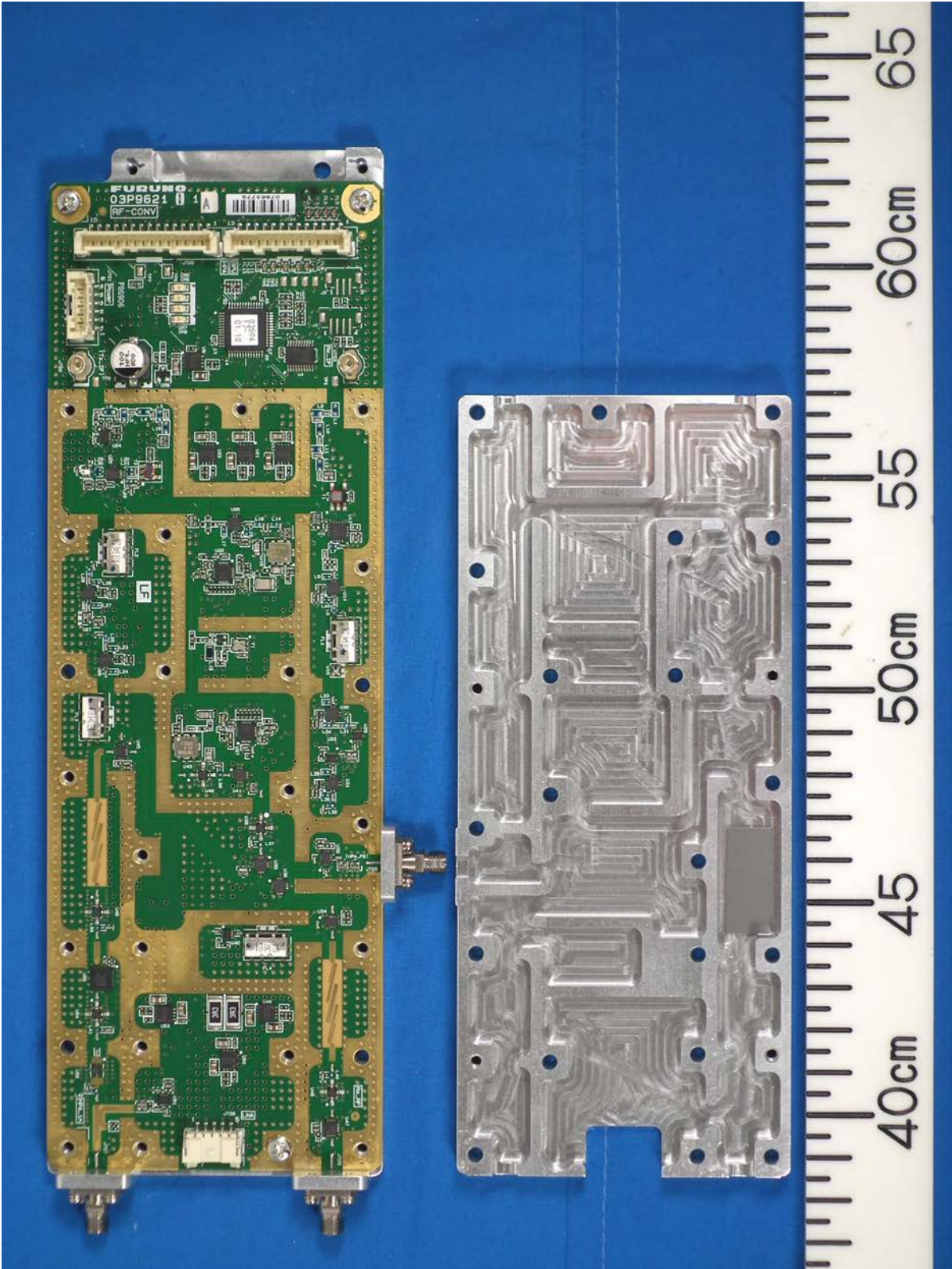
1.2.21 RF-CONV module (with the shielding cover removed, showing RF-CONV board 03P9621)
