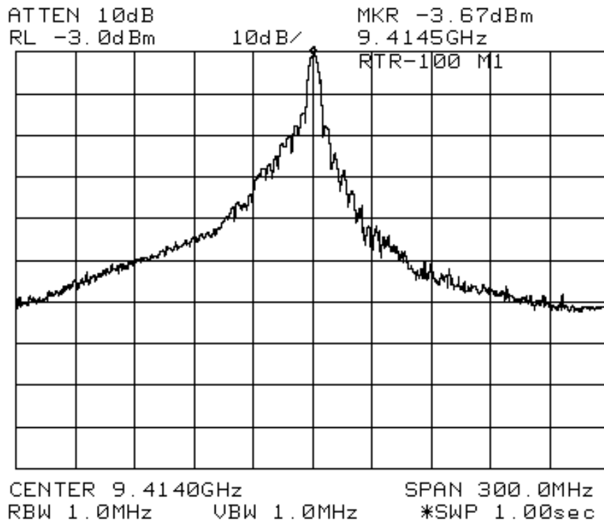
Fig. 7.3 M1 Pulse Envelope and Spectrum
