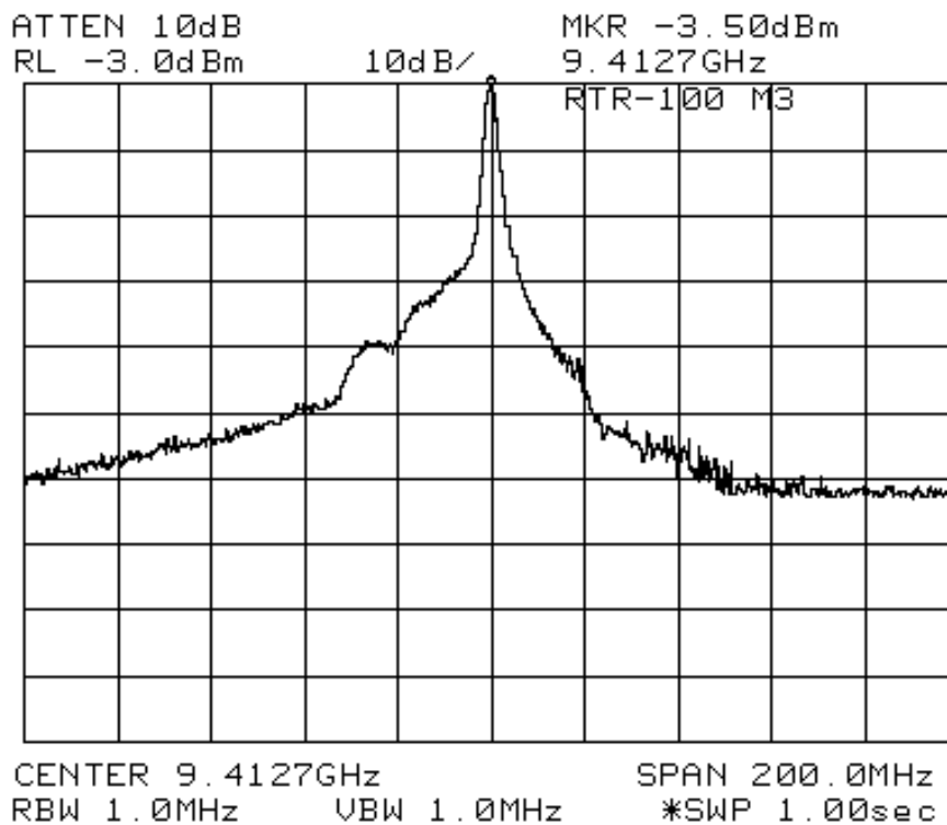
Fig. 7.5 M3 Pulse Envelope and Spectrum
