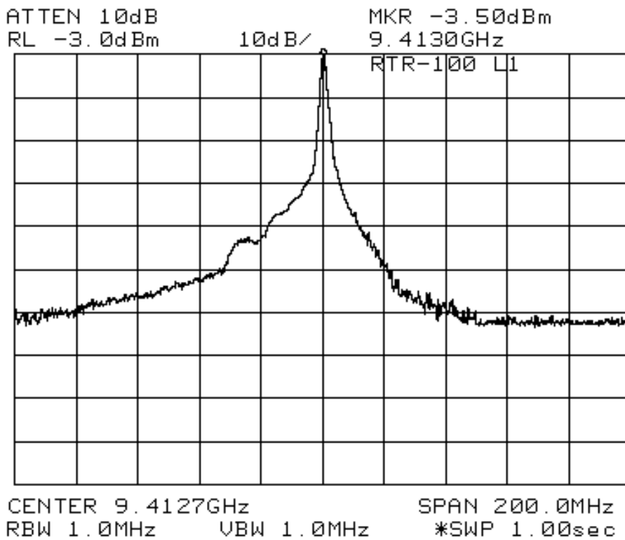
Fig. 7.6 L1 Pulse Envelope and Spectrum
