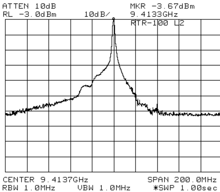
Fig. 7.7 L2 Pulse Envelope and Spectrum
