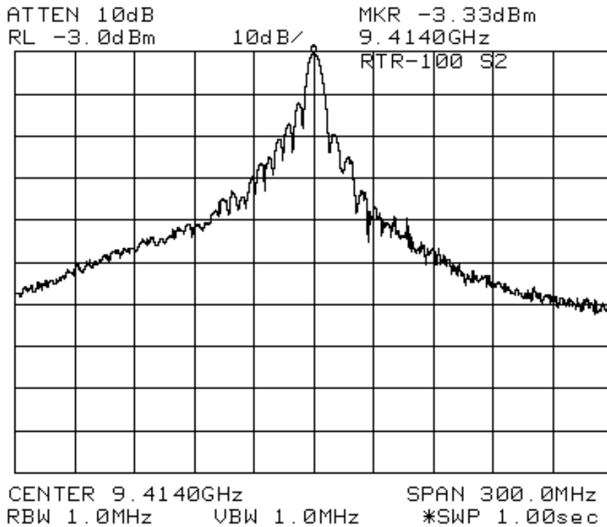
Fig. 7.2 S2 Pulse Envelope and Spectrum
