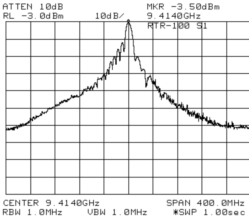
Fig. 7.1 S1 Pulse Envelope and Spectrum
