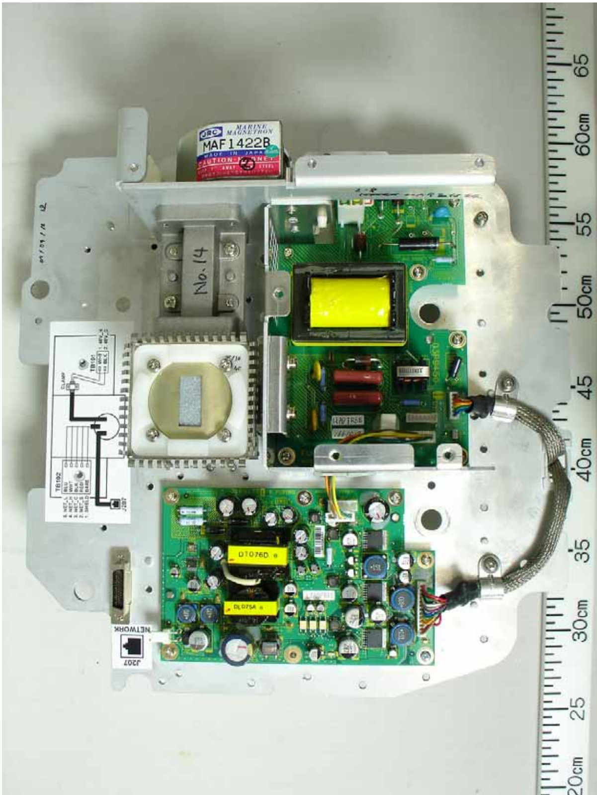
Fig. 1.1.5 Transceiver module Top View (with Shield-cover removed, showing PWR Board 03P9452 (left) and MD Board 03P9450B (right))
