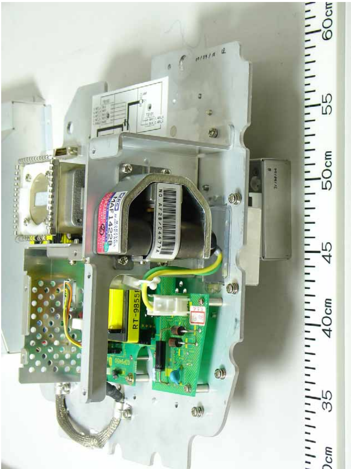
Fig. 1.1.6 Transceiver module Top View (with Shield-cover removed, showing MD Board 03P9450B (left) and Magnetron (right))
