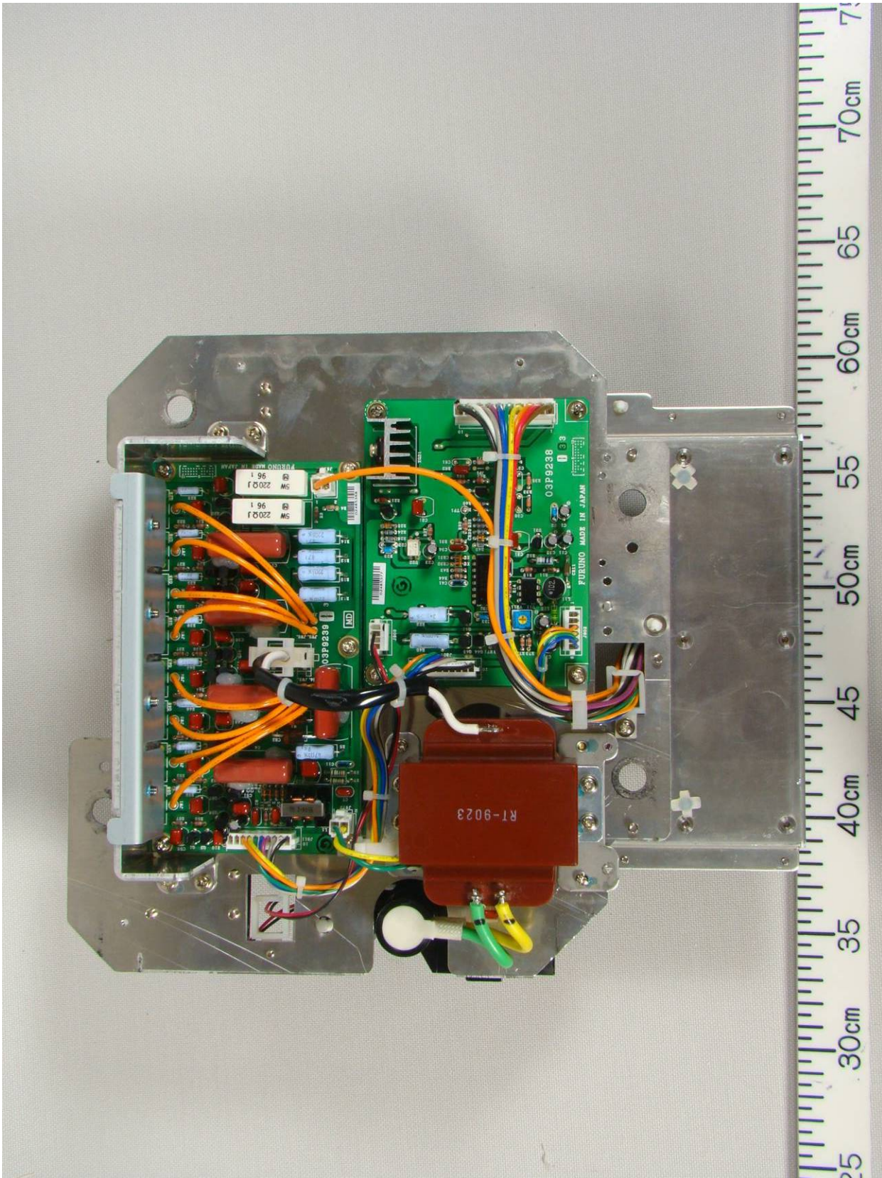
1.6 Transceiver Bottom View (with shield-cover removed, showing MD Board 03P9239 (left), RFC Board 03P9238 (upper right) and Pulse Transformer (lower right))
