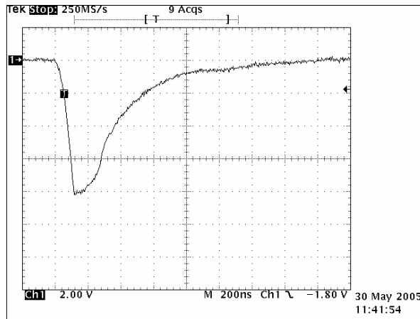
Fig. 3.2.2.1 Short Pulse (0.125 nm Range) Scale: 2 kV/div. 200 ns/div.
