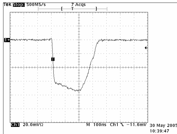
Fig. 3.2.3.3 Middle Pulse (1.5 nm Range) Scale: 20 mV/div. 100 ns/div.
