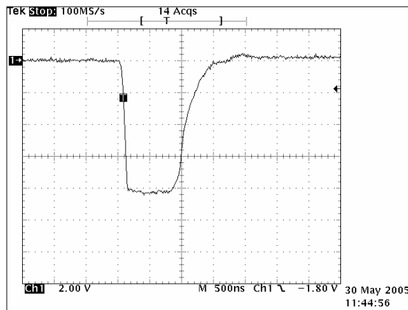
Fig. 3.2.2.3 Long 1 Pulse (3 nm Range) Scale: 2 kV/div. 500 ns/div.
