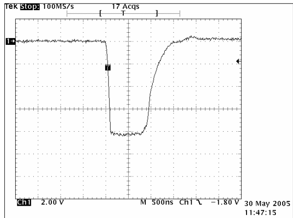
Fig. 3.2.2.5 Long 3 Pulse (96 nm Range) Scale: 2 kV/div. 500 ns/div.
