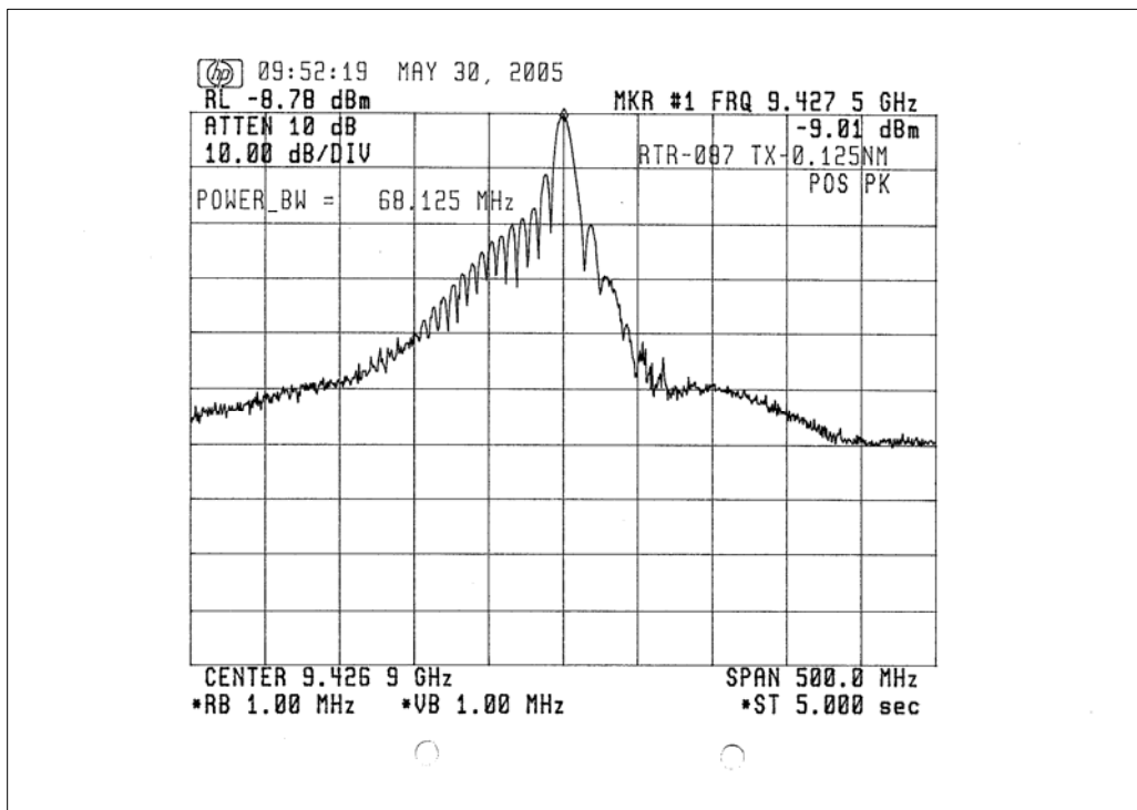
Fig. 3.3.2 Measurement of Occupied Bandwidth
