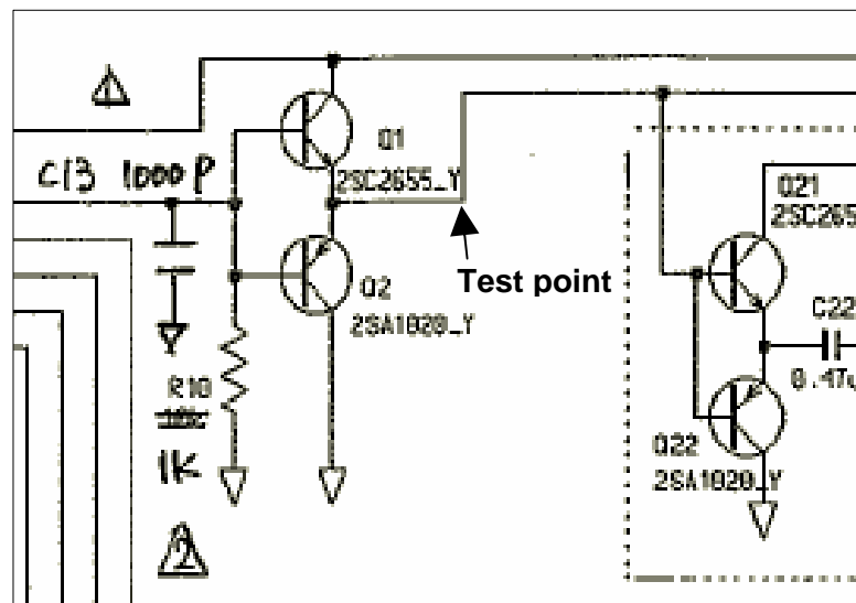
Fig. 3.2.1.2 Test Point for Trigger Pulse (in MD board (03P9239) of Radar Antenna Unit)
