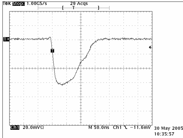
Fig. 3.2.3.2 Short Pulse (0.125 nm Range) Scale: 20 mV/div. 50 ns/div.
