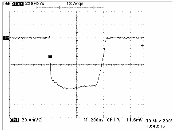
Fig. 3.2.3.6 Long 3 Pulse (96 nm Range) Scale: 20 mV/div. 200 ns/div.
