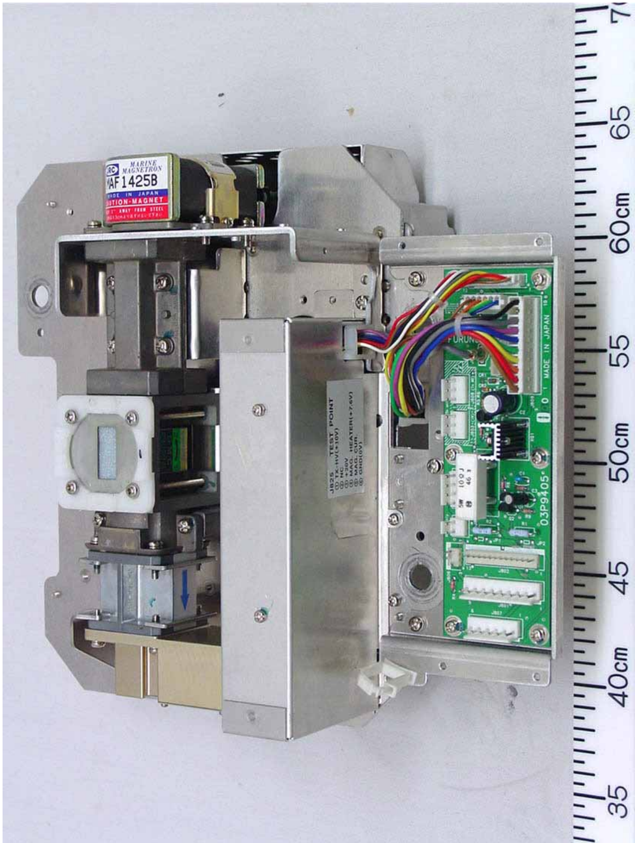
1.1.2 Transceiver Top View (with RTB shield-cover removed, showing RTB Board 03P9405 (right), IF AMP Board enclosed by shield-cover (center), Magnetron (top left), Circulator (center left), Limiter (lower left) and MIC (bottom left))
