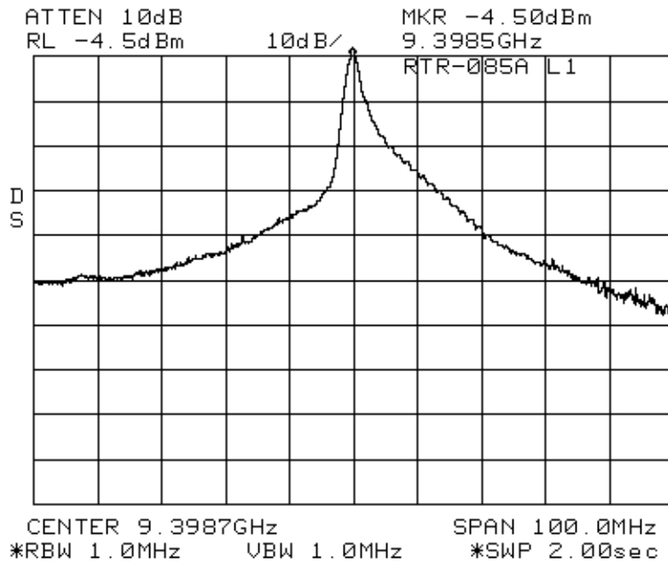
Fig. 7.3 L1 Pulse Envelope and Spectrum
