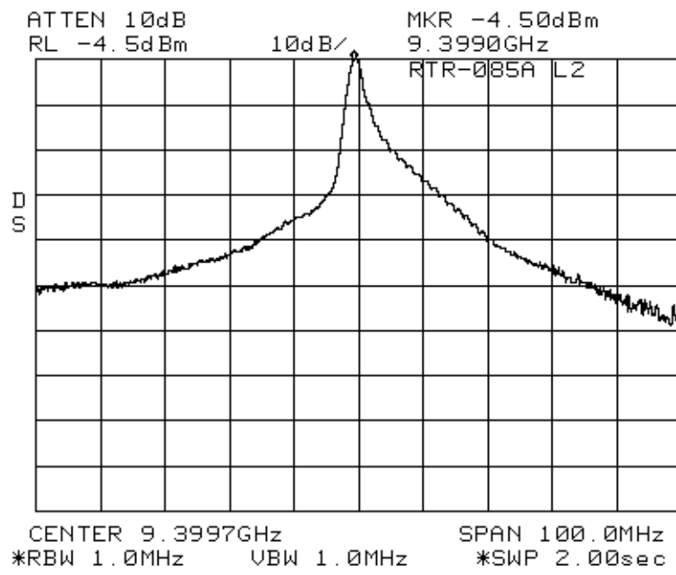
Fig. 7.4 L2 Pulse Envelope and Spectrum
