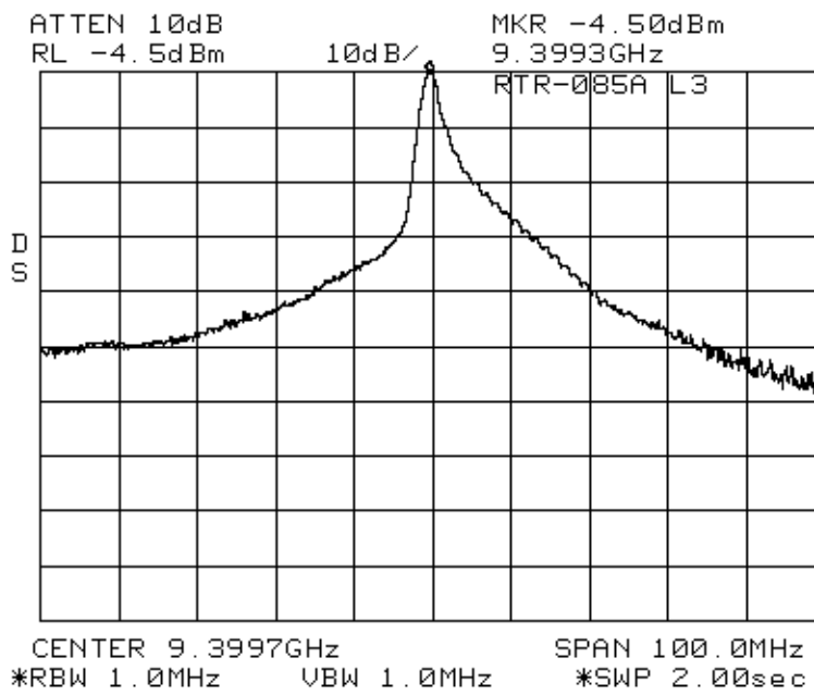
Fig. 7.5 L3 Pulse Envelope and Spectrum
