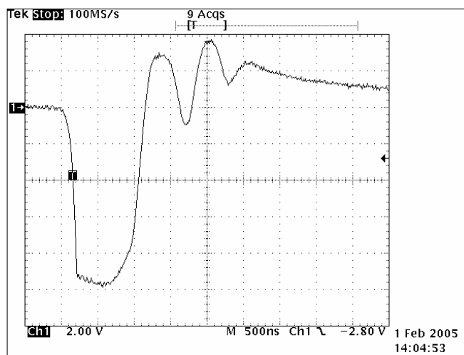
Fig. 3.2.2.3 Middle 2 Pulse (12 nm Range) Scale: 2 kV/div. 500 ns/div.
