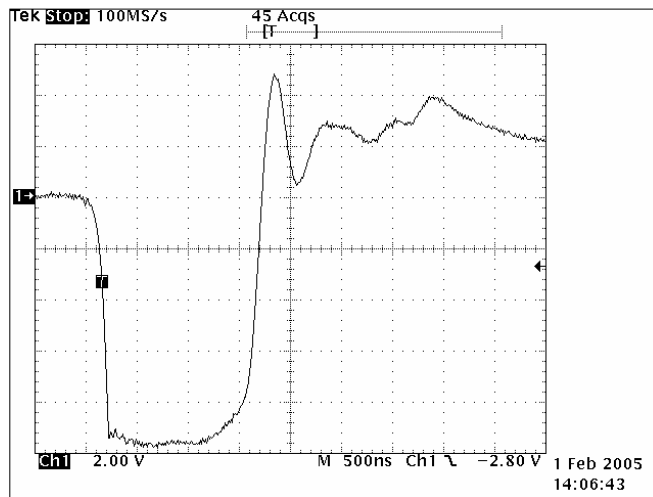
Fig. 3.2.2.4 Long 1 Pulse (48 nm Range) Scale: 2 kV/div. 500 ns/div.
