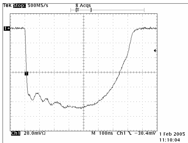
Fig. 3.2.3.4 Middle 2 Pulse (12 nm Range) Scale: 20 mV/div. 100 ns/div.
