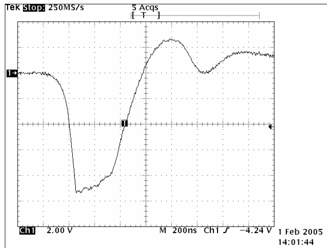
Fig. 3.2.2.2 Middle 1 Pulse (3 nm Range) Scale: 2 kV/div. 200 ns/div.
