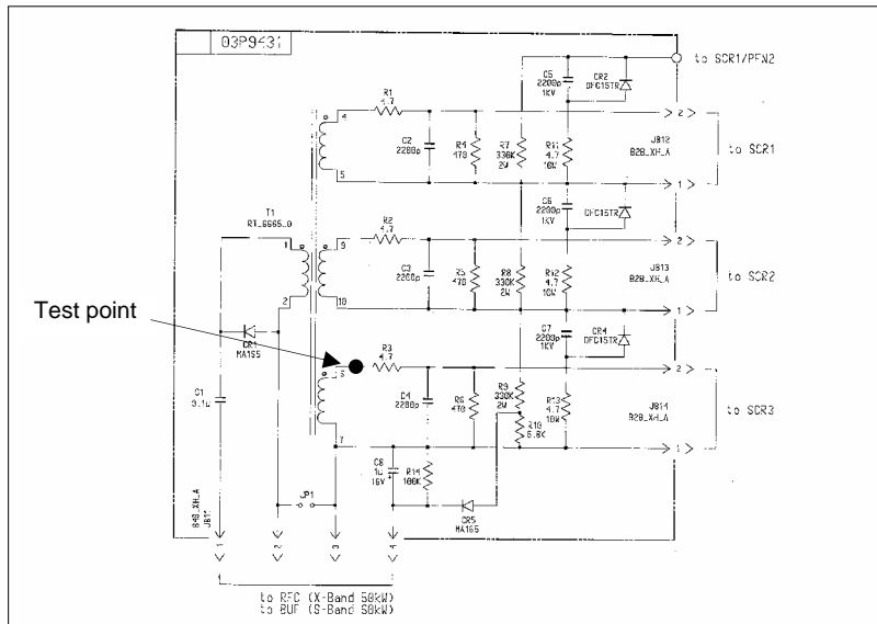
Fig. 3.2.1.2 Test Point for observing Trigger Pulse (in MD board (03P9431) of Radar Antenna Unit)
