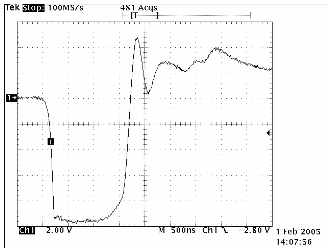
Fig. 3.2.2.5 Long 2 Pulse (96 nm Range) Scale: 2 kV/div. 500 ns/div.
