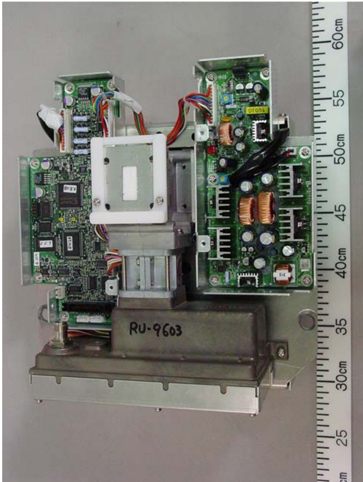
1.5 Transceiver module Top View (showing RFC Board 03P9346 (left) and PWR Board 03P9348 (right))
