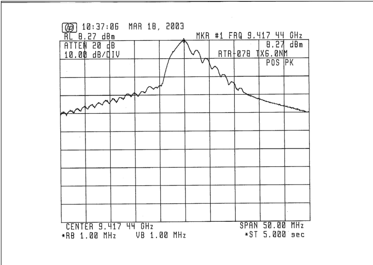
Fig. 3.2.4.4 For Middle 2 Pulse (6 nm Range)
