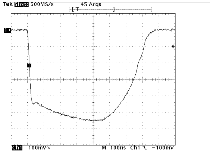
Fig. 3.2.3.5 Middle 2 Pulse (6 nm Range) Scale: 100 mV/div. 100 ns/div.
