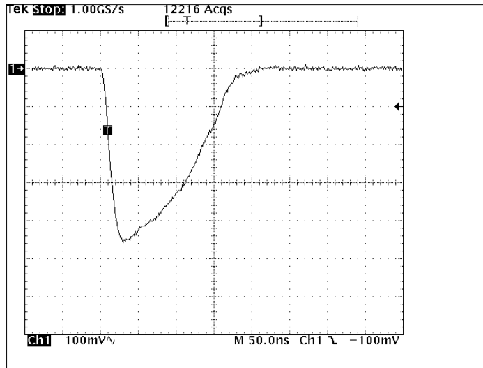
Fig. 3.2.3.2 Short 1 Pulse (0.125 nm Range) Scale: 100 mV/div. 50 ns/div.
