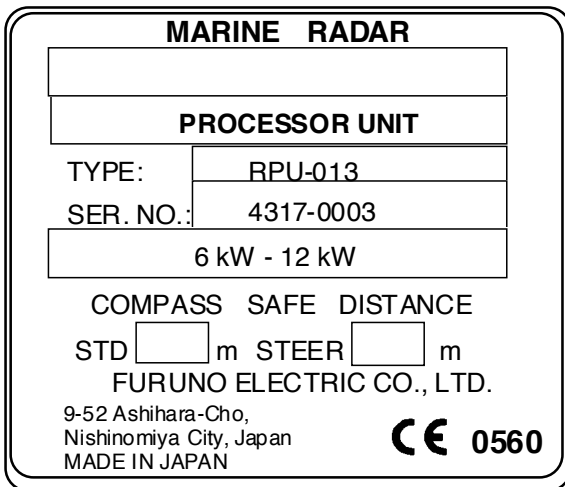
Fig. 2.2 Nameplate for Processor Unit
