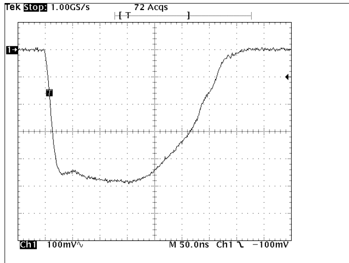
Fig. 3.2.3.3 Short 2 Pulse (1.5 nm Range) Scale: 100 mV/div. 50 ns/div.
