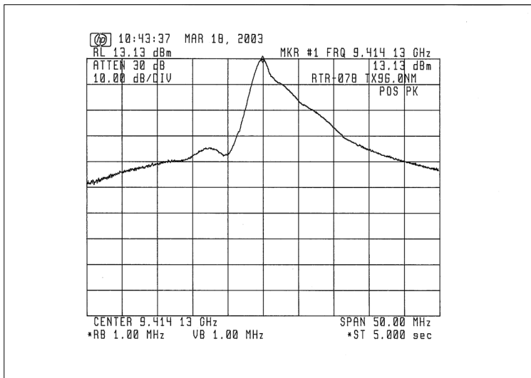
Fig. 3.2.4.7 For Long 2 Pulse (96 nm Range)
