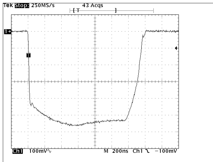
Fig. 3.2.3.7 Long 1 Pulse (48 nm Range) Scale: 100 mV/div. 200 ns/div.
