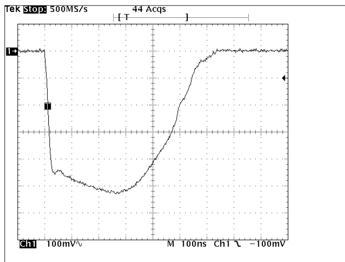
Fig. 3.2.3.4 Middle 1 Pulse (3 nm Range) Scale: 100 mV/div. 100 ns/div.
