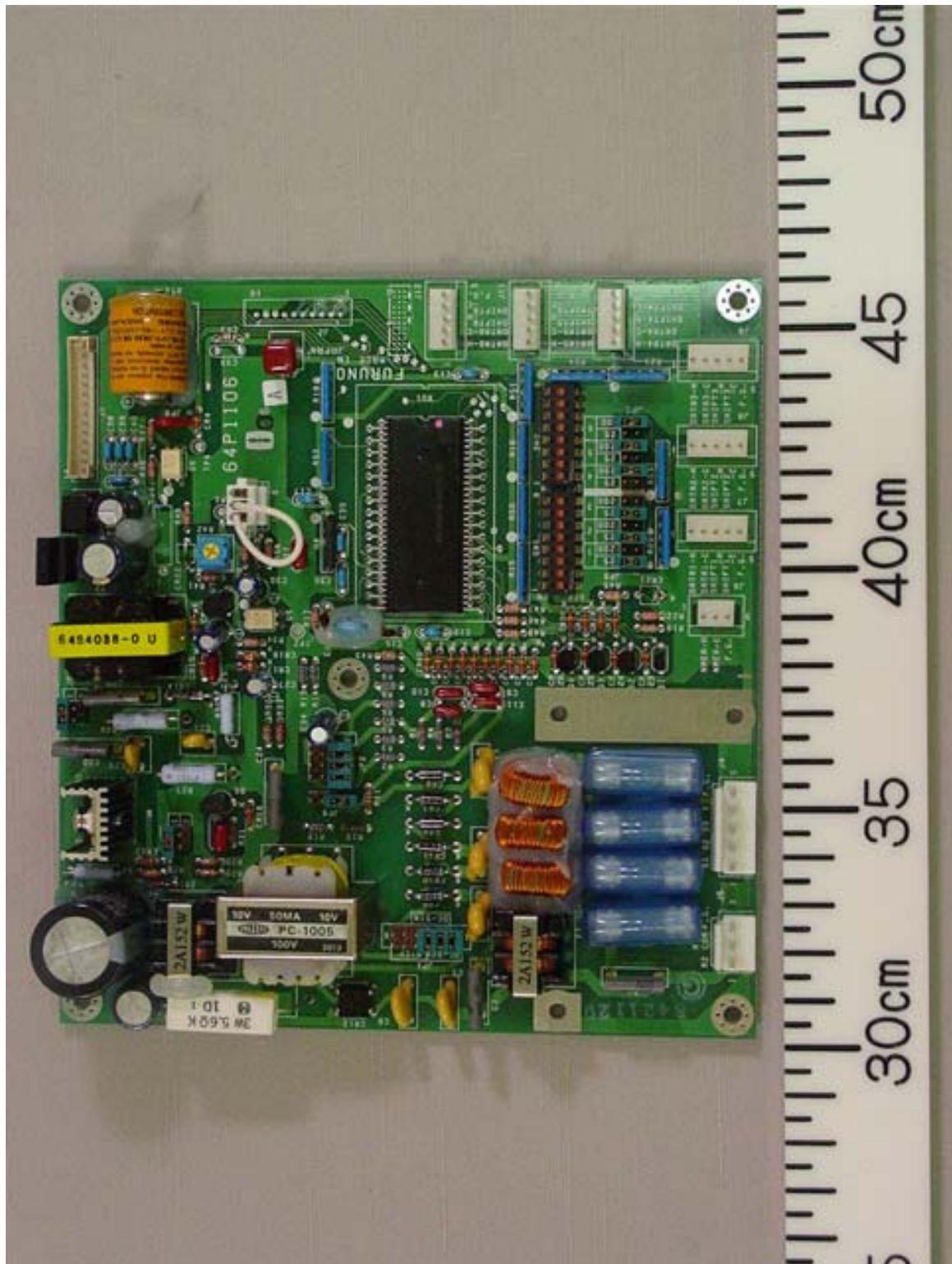
2.16 GC-10 Board 16P1106 Front side
