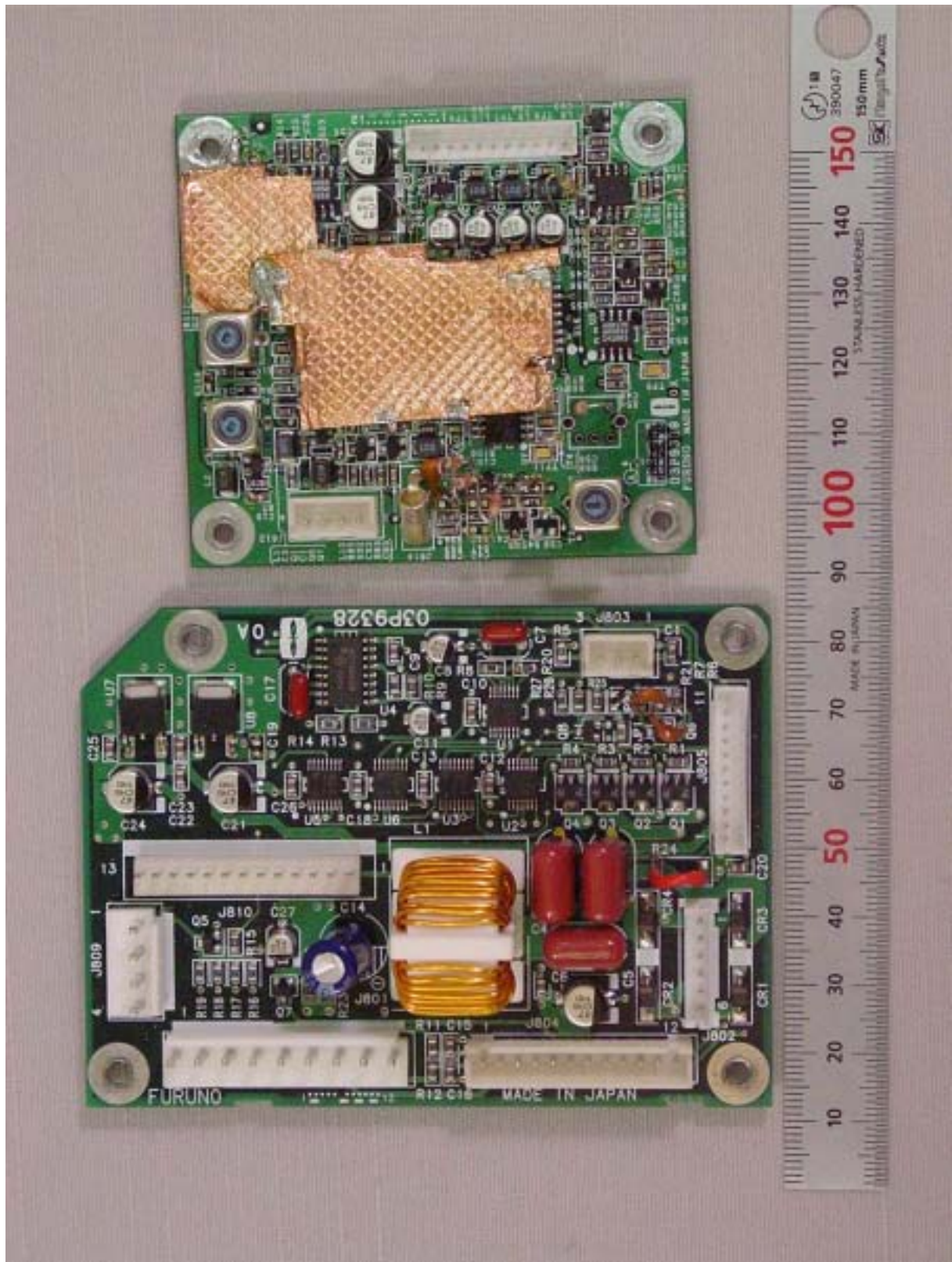
1.6 IF 03P9329 (upper) and INT 03P9328 (lower) Boards Front side
