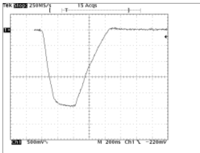
Middle Pulse (2 nm Range)
