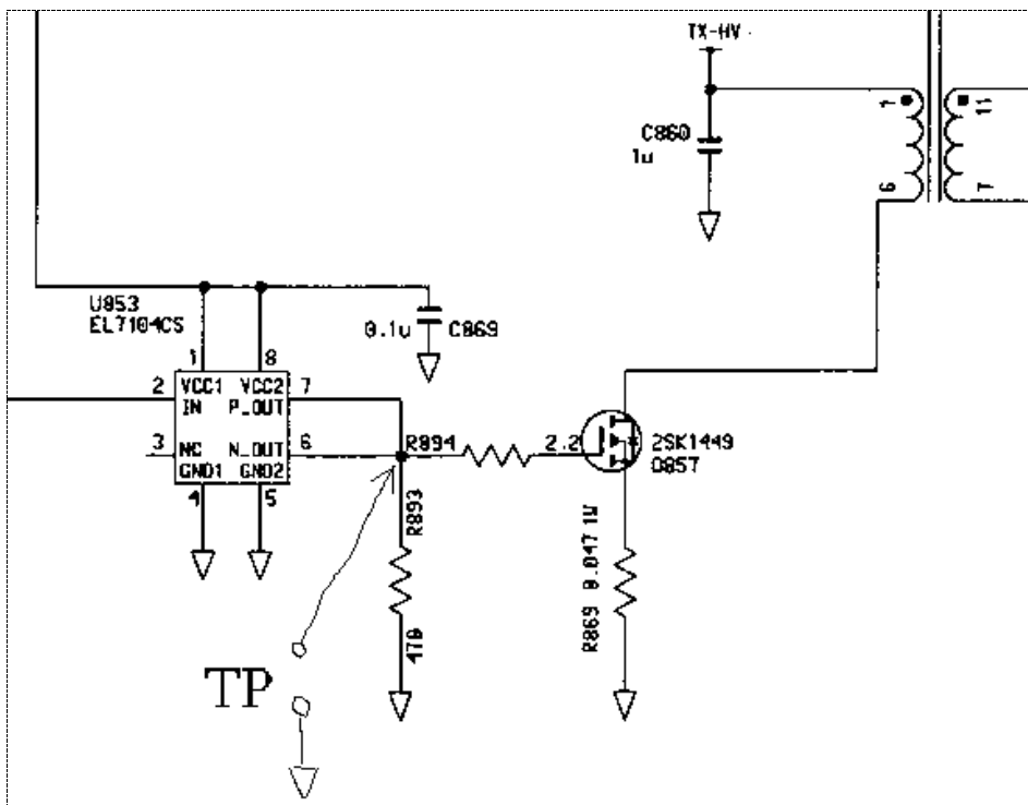
Fig. 3.2.1.2 Test Point for Trigger Pulse (in MD Board (03P9270) of Radar Antenna Unit)
