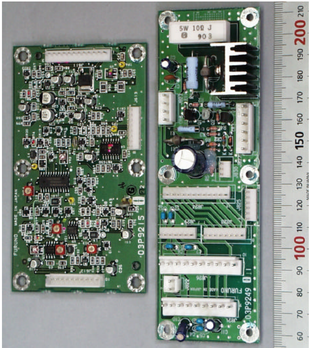
Fig. 2.7 IF Board 03P9215 (left) and TB & Motor Starter Board 03P9249 (right)
