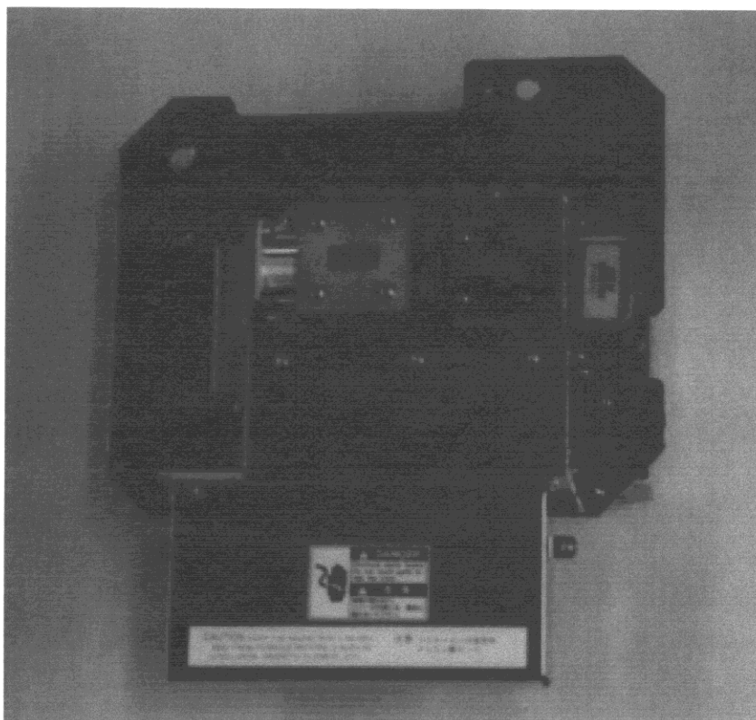
Photo 10.13 Transceiver Module (RTR-059) Top View (showing Magnetron and Circulator)
