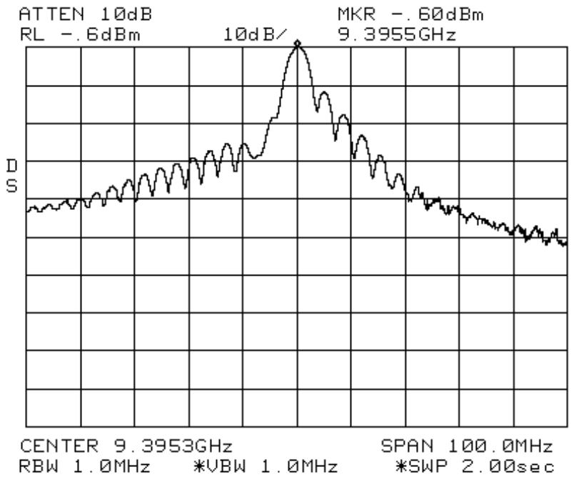
Fig. 7.2 M Pulse Envelope and Spectrum
