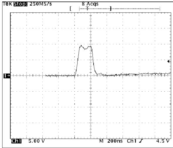
Typical waveform of Trigger Pulse
