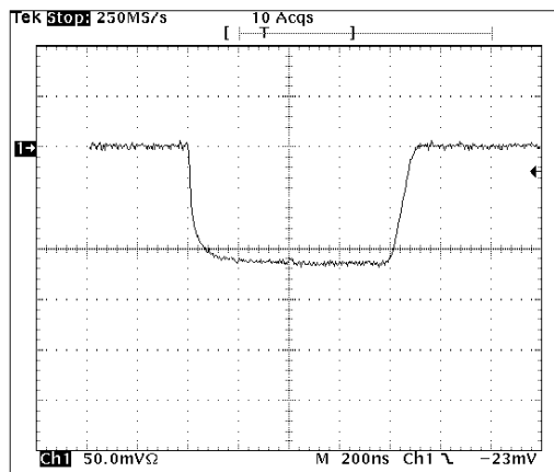
Long Pulse (36 nm Range)
