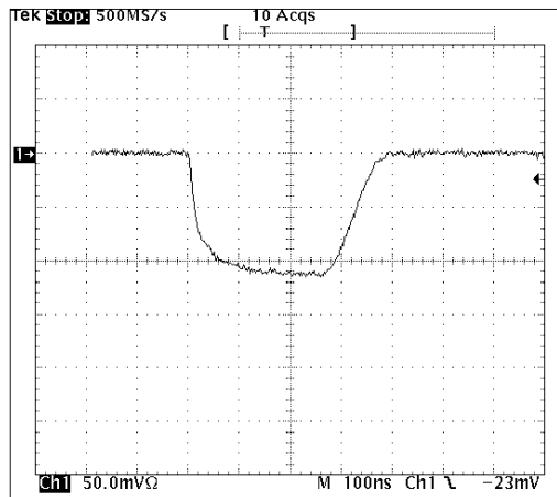
Middle Pulse (2 nm Range)
