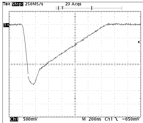
Short Pulse (0.25 nm Range)
