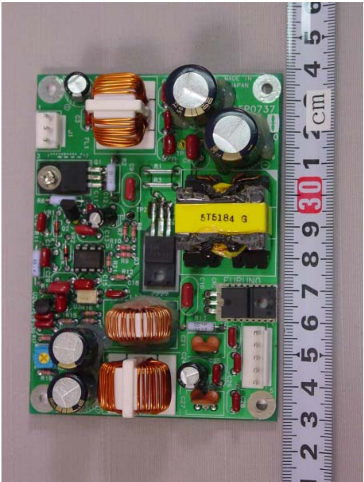
A.21 SW-REG Board 05P0737 Front side
