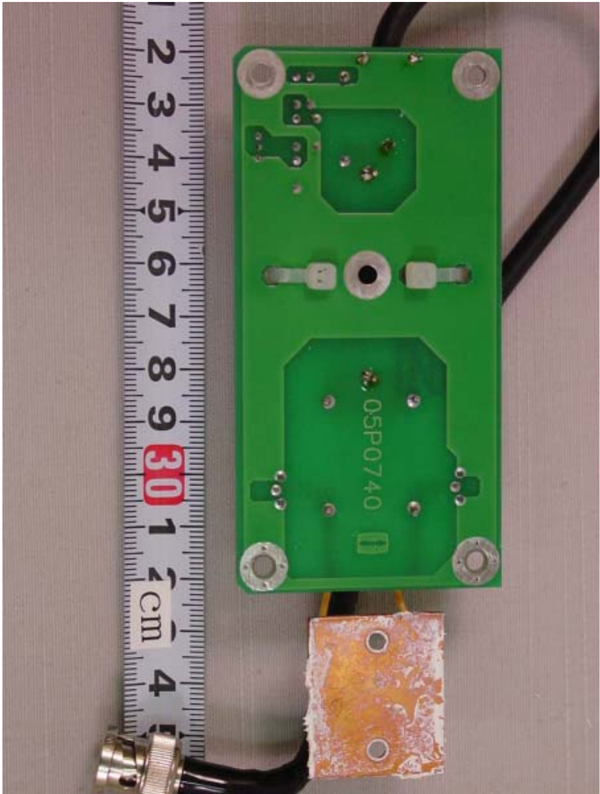
A.18 COMB Board 05P0740 Rear side
