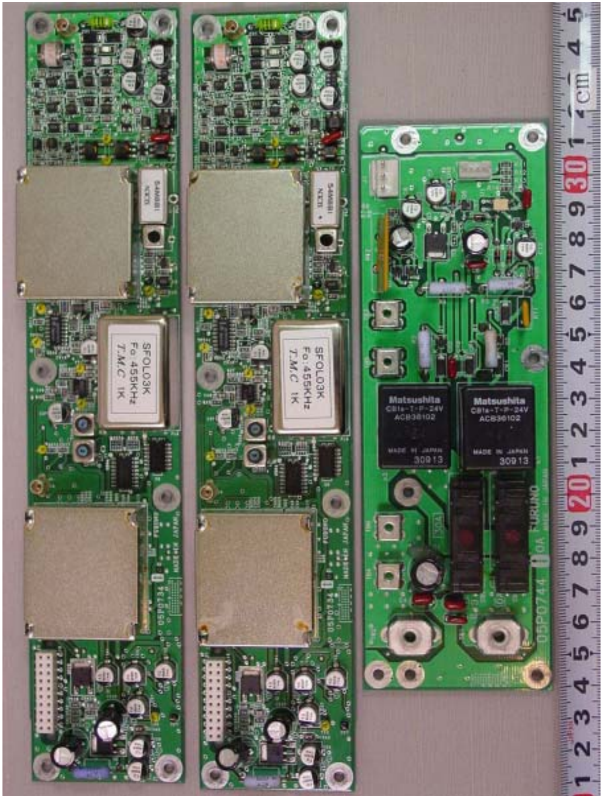
A.11 W/R Boards 05P0734 (left & center) and RELAY Board 05P0744 (right) Front side
