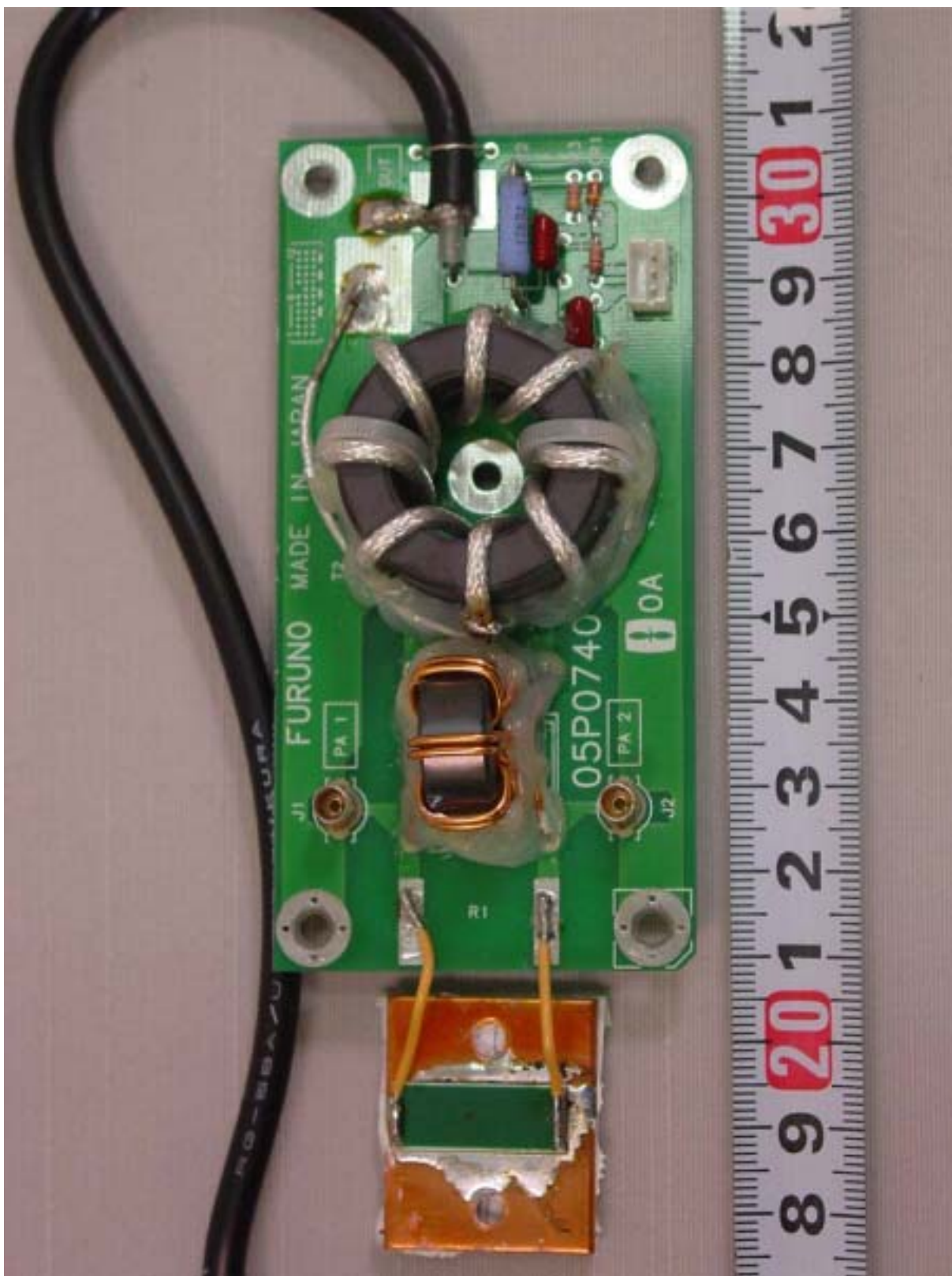
A.17 COMB Board 05P0740 Front side
