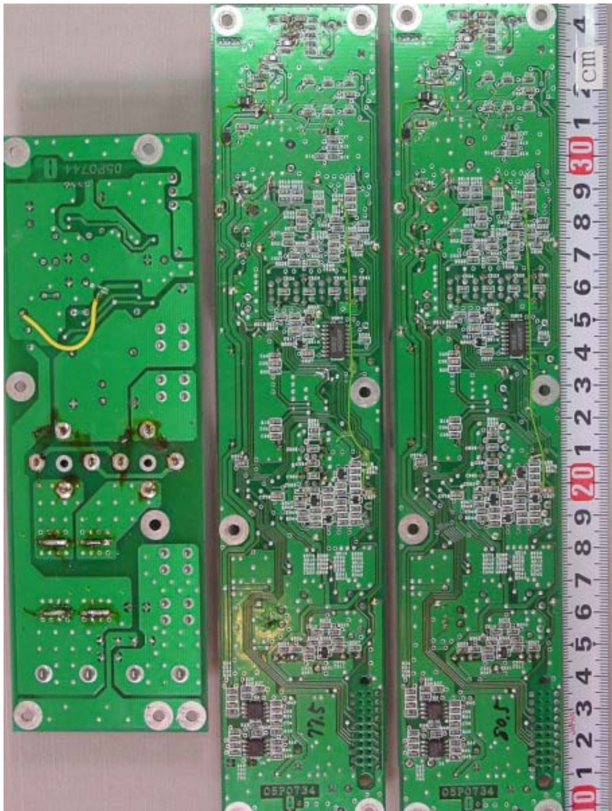
A.12 W/R Boards 05P0734 (right & center) and RELAY Board 05P0744 (left) Rear side
