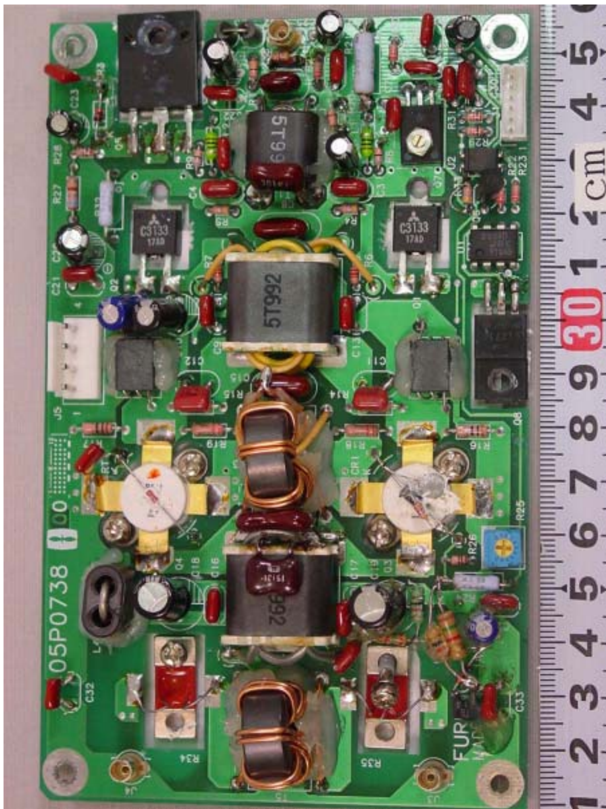
A.13 DRV Board 05P0738 Front side
