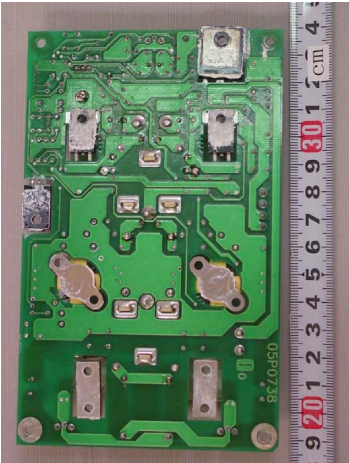
A.14 DRV Board 05P0738 Rear side
