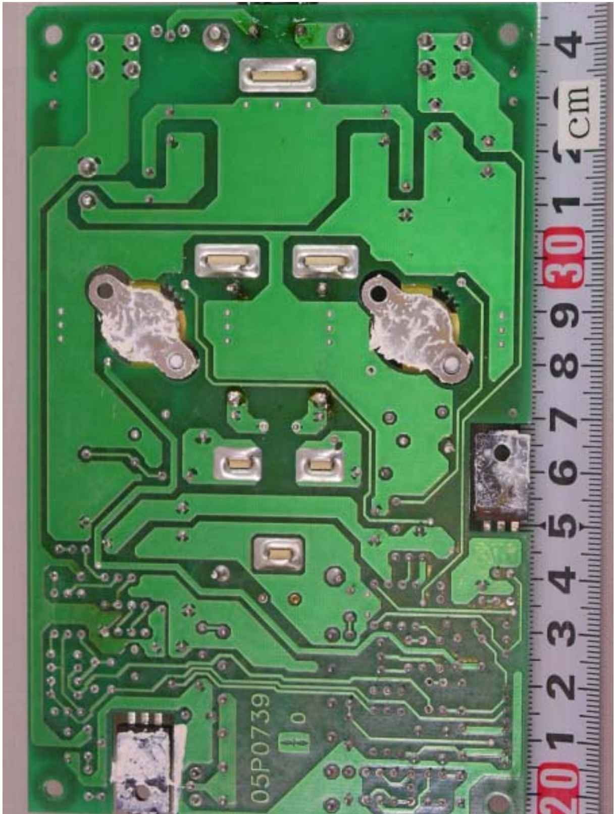
A.16 PA Board 05P0739 Rear side
