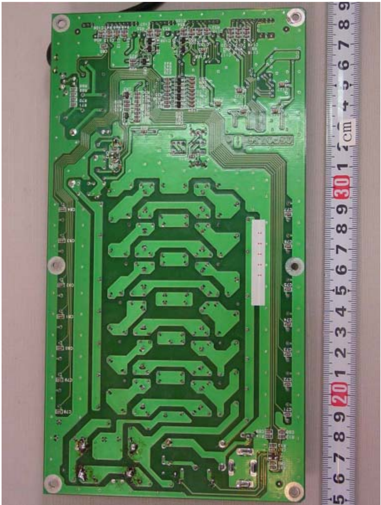
A.20 TX-FIL Board 05P0736 Rear side
