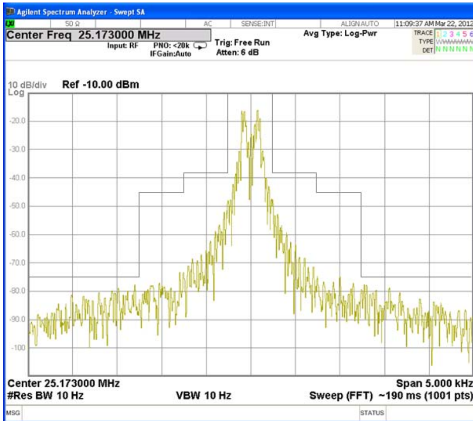
Fig. 3.3.30 NBDP(FEC): Tx Frequency 25173 kHz
