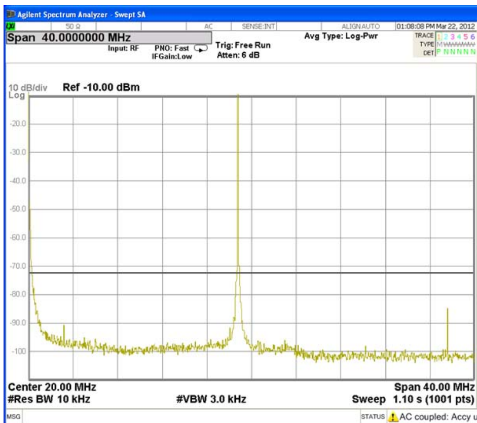
Fig. 3.5.17 Tx Frequency 18780 kHz
