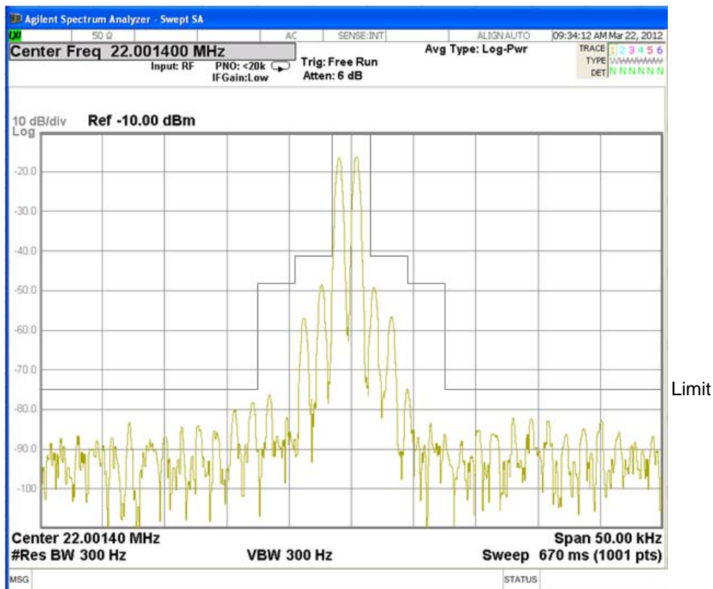
Fig. 3.4.11 SSB: Tx Frequency 22000 kHz
