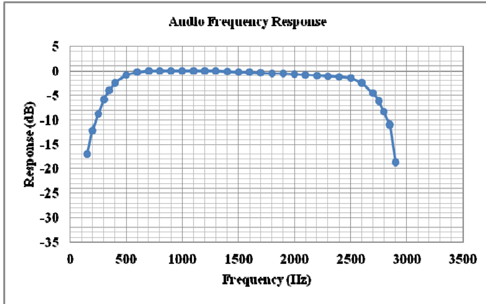
Fig. 3.2.2 Audio Frequency Response
