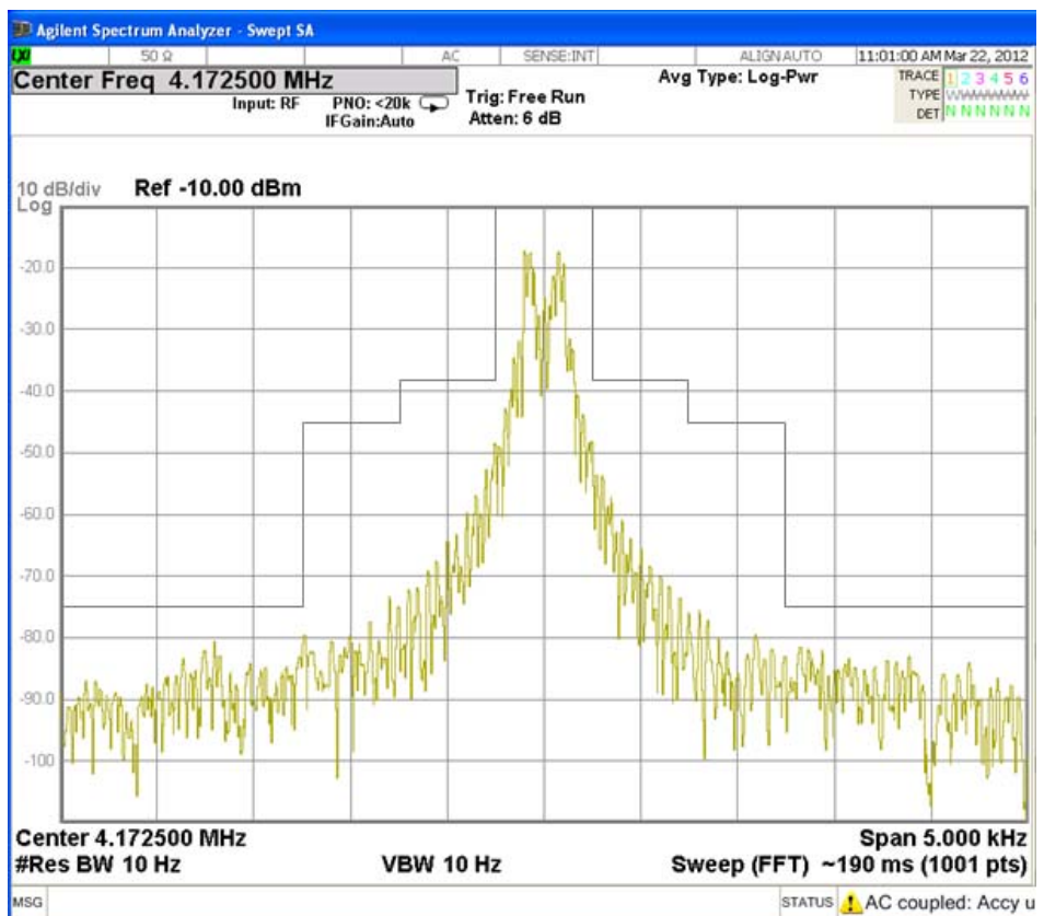
Fig. 3.3.23 NBDP(FEC): Tx Frequency 4172.5 kHz
