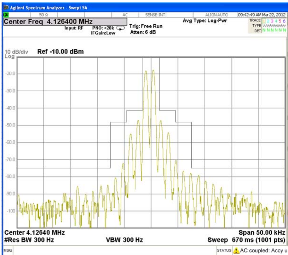
Fig. 3.3.5 SSB: Tx Frequency 4125 kHz
