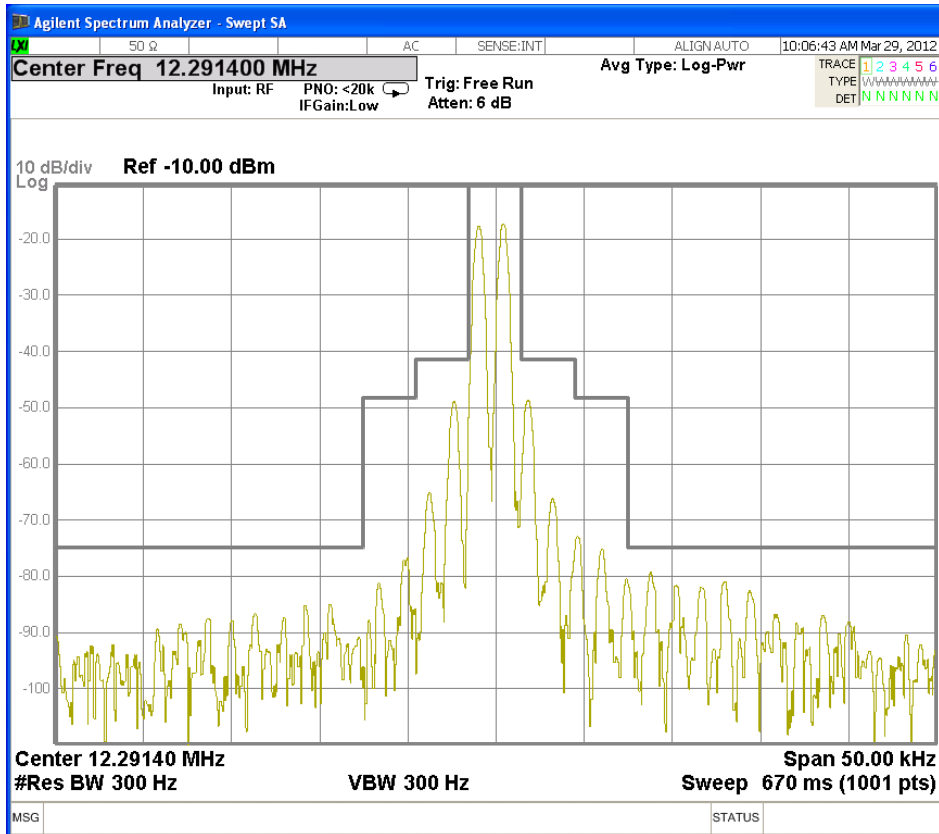
Fig. 3.3.8 SSB: Tx Frequency 12290 kHz
