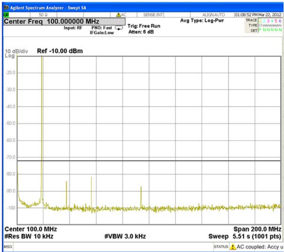
Fig. 3.5.18 Tx Frequency 18780 kHz
