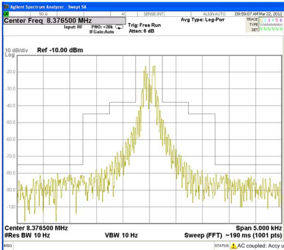
Fig. 3.3.16 NBDP(ARQ): Tx Frequency 8376.5 kHz
