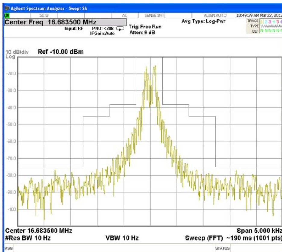
Fig. 3.3.27 NBDP(FEC): Tx Frequency 16683.5 kHz
