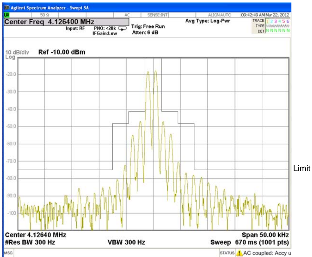
Fig. 3.4.5 SSB: Tx Frequency 4125 kHz
