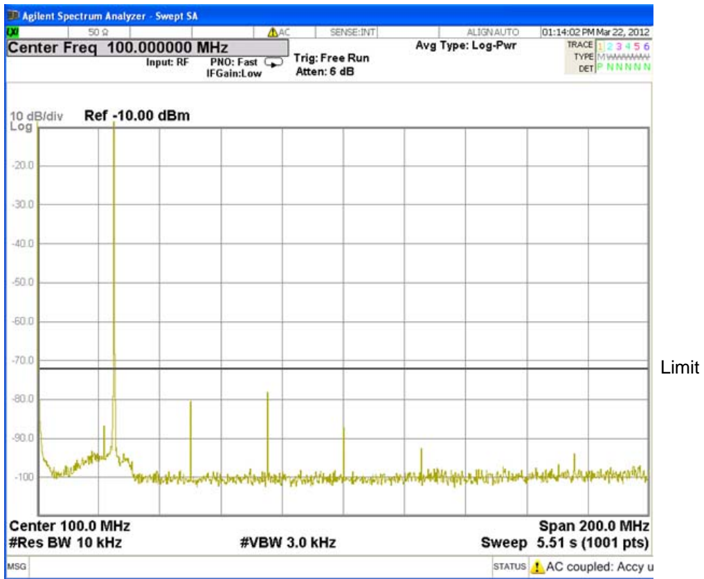
Fig. 3.5.22 Tx Frequency 25070 kHz
