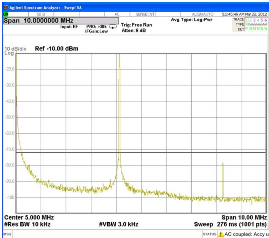
Fig. 3.5.7 Tx Frequency 4125 kHz
