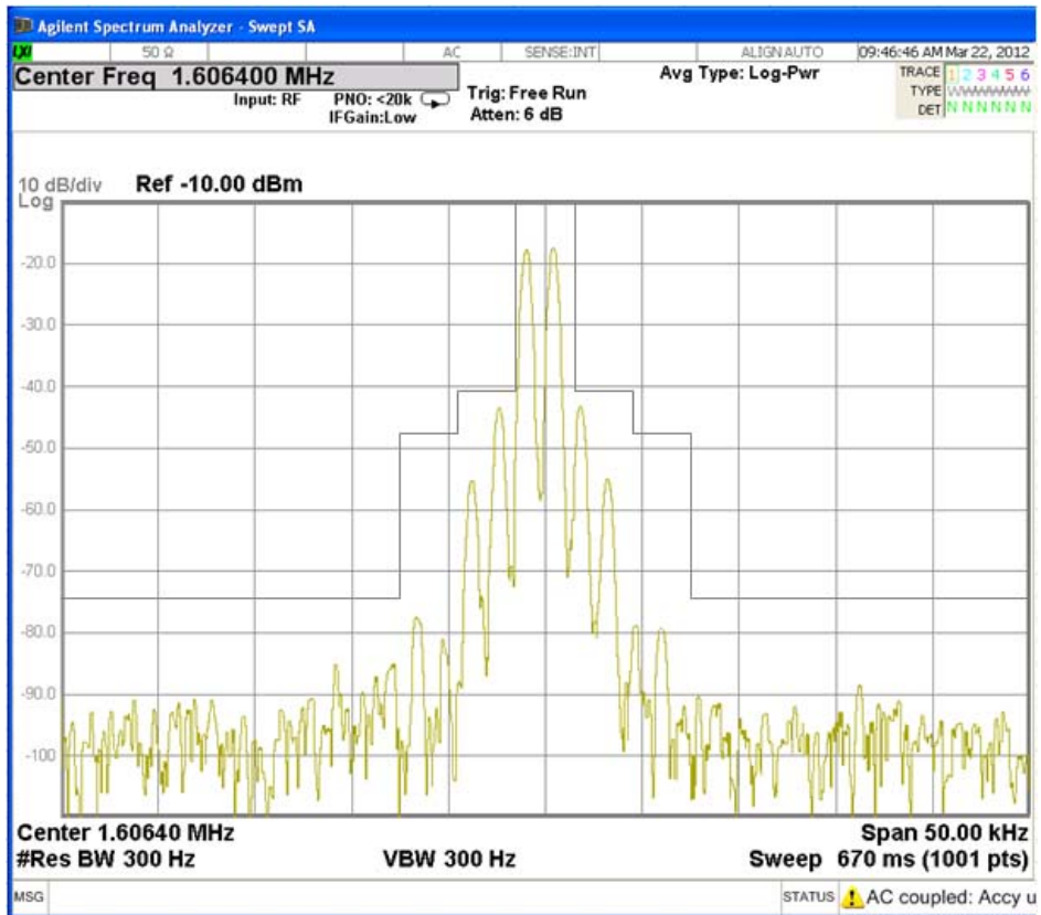
Fig. 3.3.2 SSB: Tx Frequency 1605 kHz
