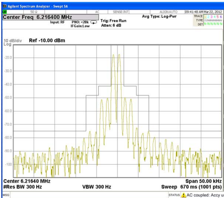
Fig. 3.4.6 SSB: Tx Frequency 6215 kHz
