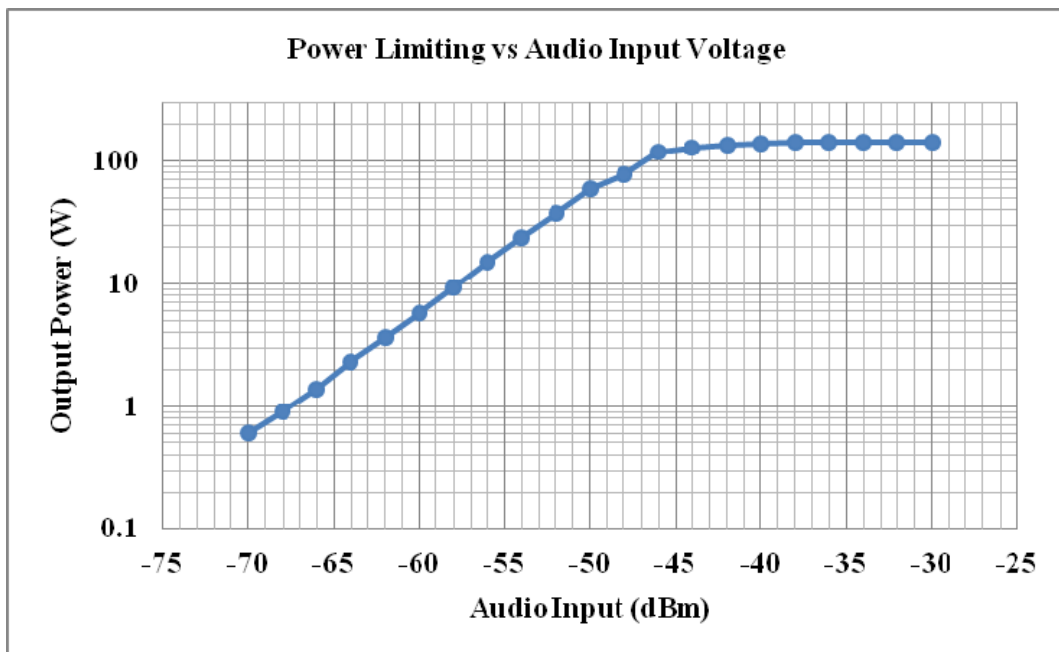
Fig. 3.2.3 Power Limiting vs Audio Input Level
