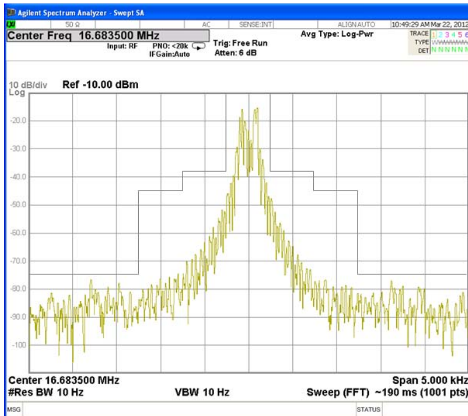
Fig. 3.3.18 NBDP(ARQ): Tx Frequency 16683.5 kHz
