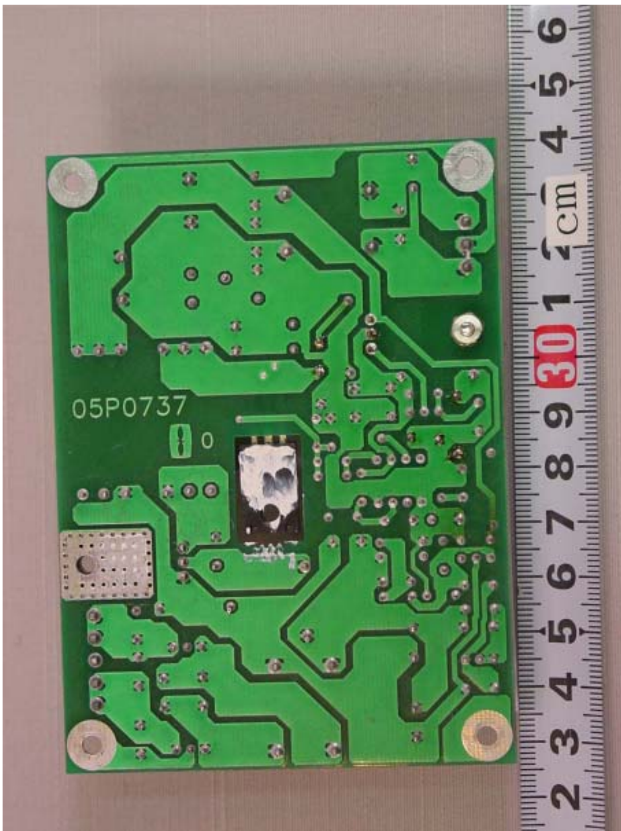
A.18 SW-REG Board 05P0737 Rear side
