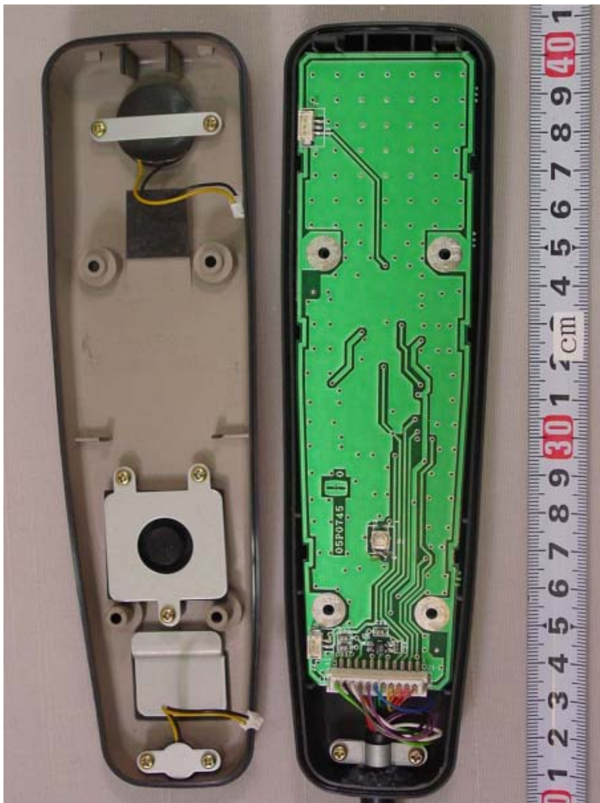
D.3 Inside View (with Cover opened, showing PCB 05P0745)
