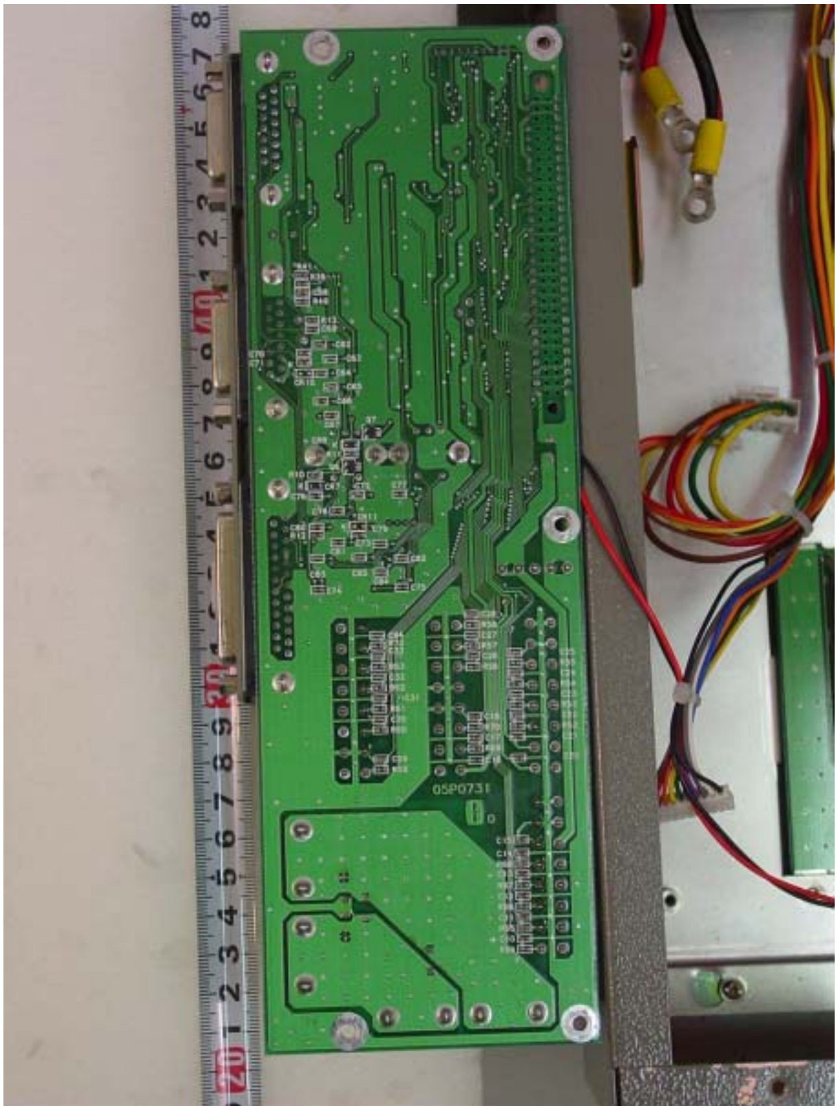
A.8 T-IF Board 05P0731 Rear side
