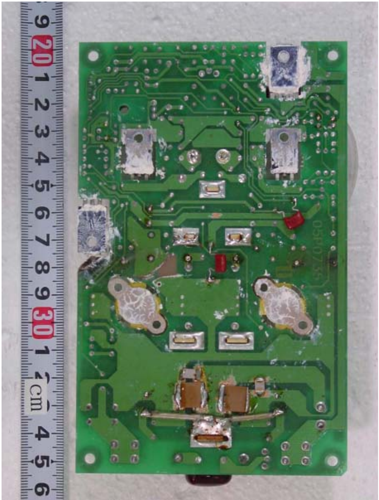
A.14 PA Board 05P0735 Rear side
