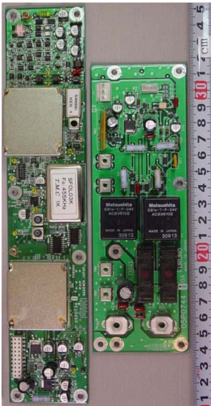
A.11 W/R Board 05P0734 (left) and RELAY Board 05P0744 (right) Front side
