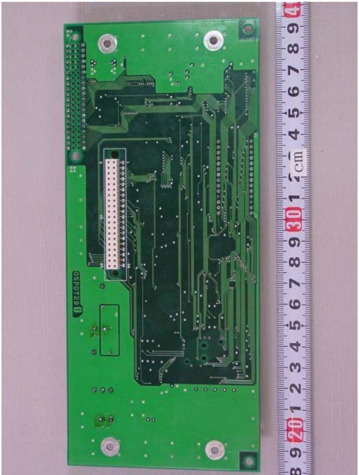
C.9 CPU Board 05P0729 Rear side
