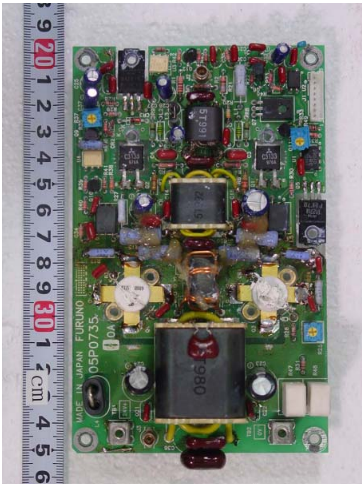
A.13 PA Board 05P0735 Front side
