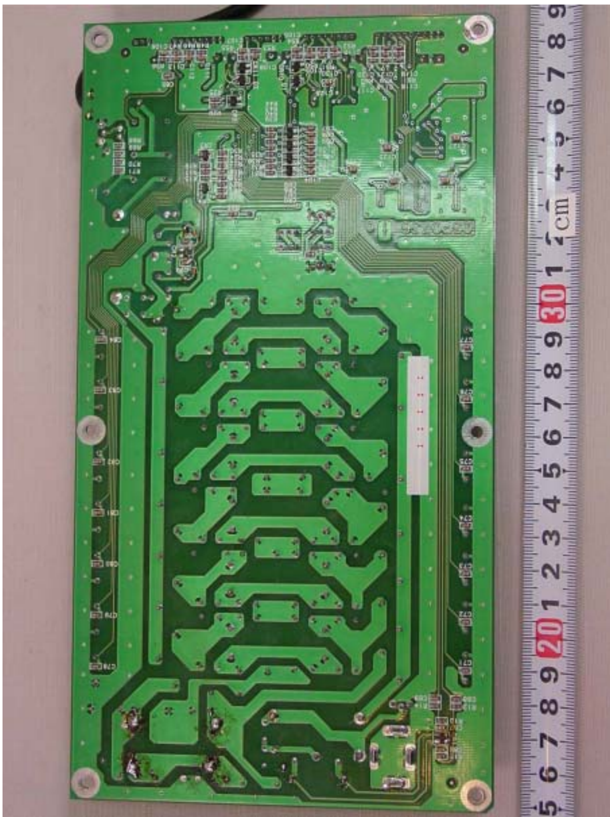
A.16 TX-FIL Board 05P0736 Rear side
