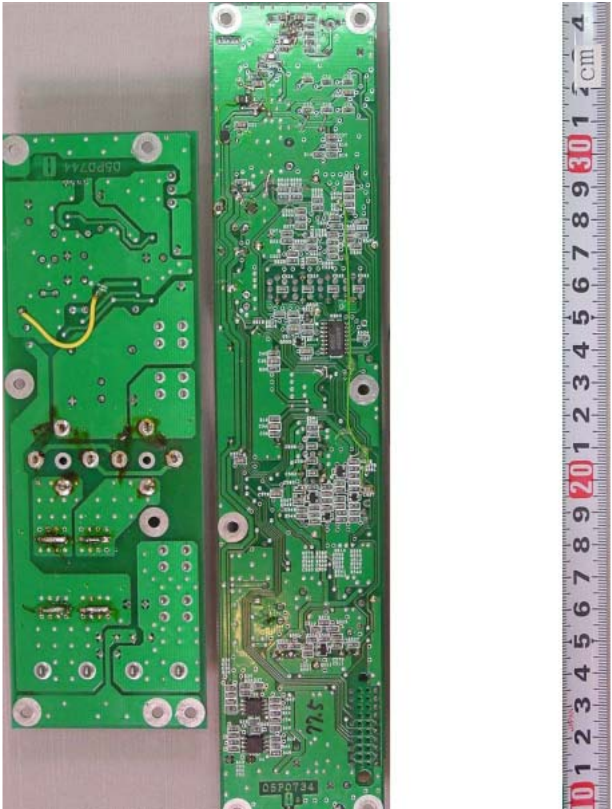
A.12 W/R Board 05P0734 (right) and RELAY Board 05P0744 (left) Rear side
