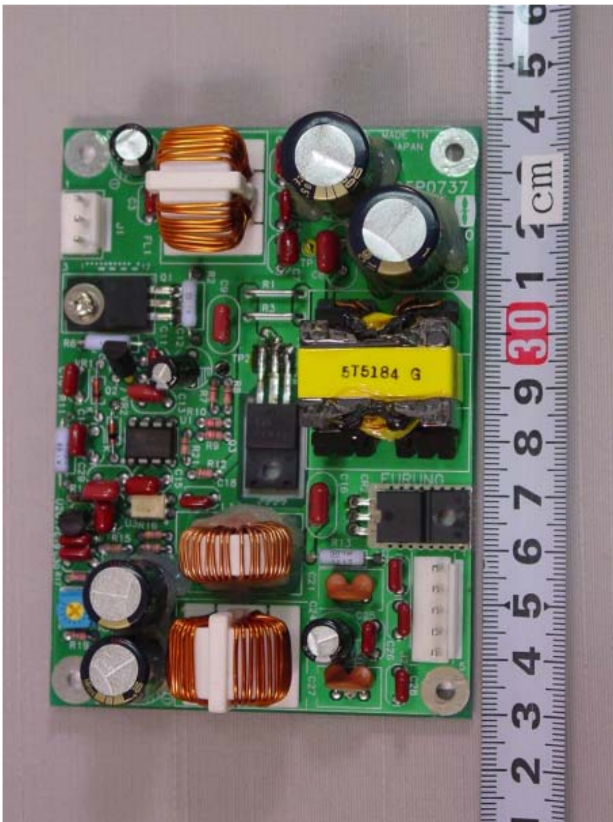
A.17 SW-REG Board 05P0737 Front side
