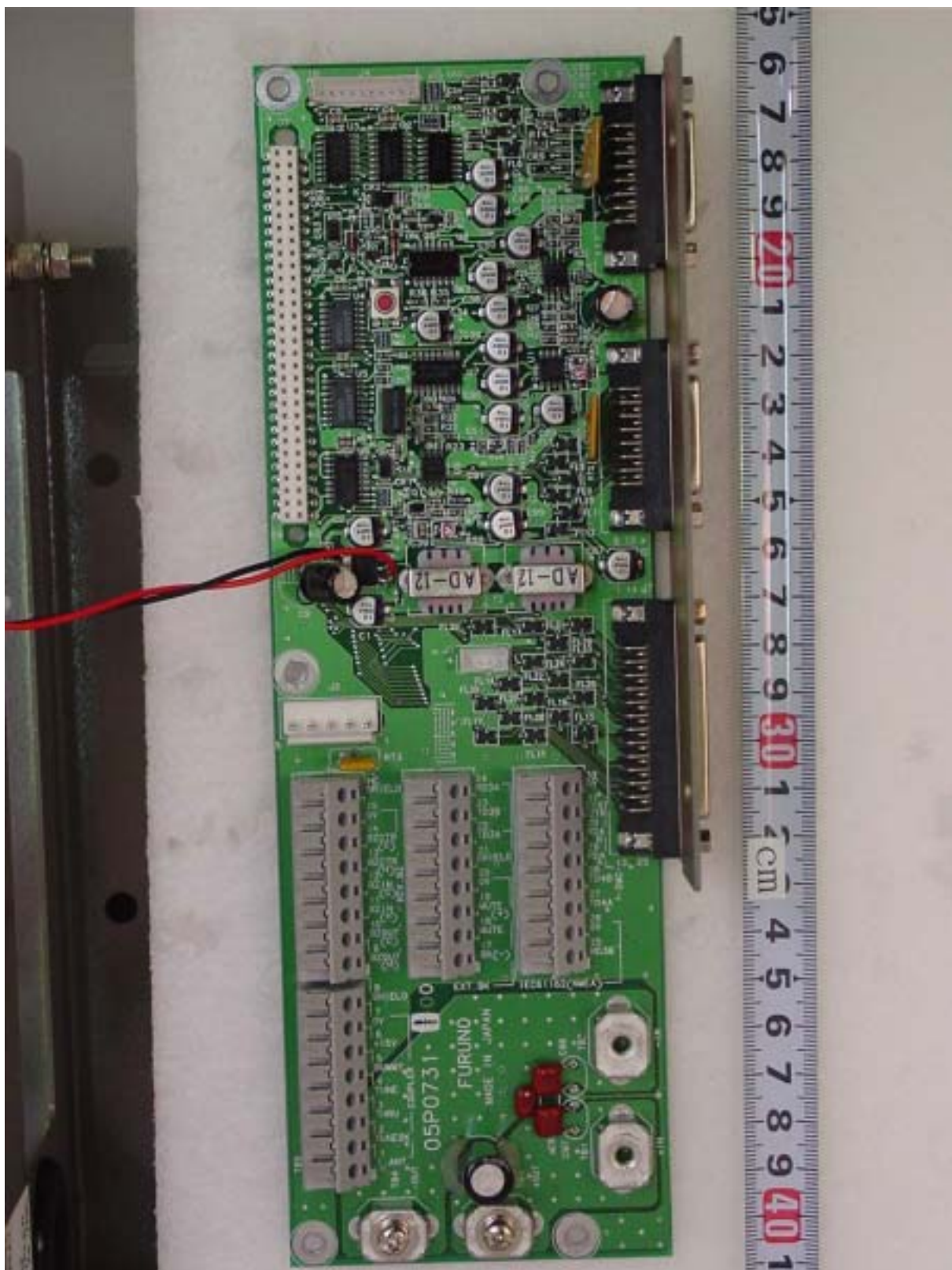
A.7 T-IF Board 05P0731 Front side
