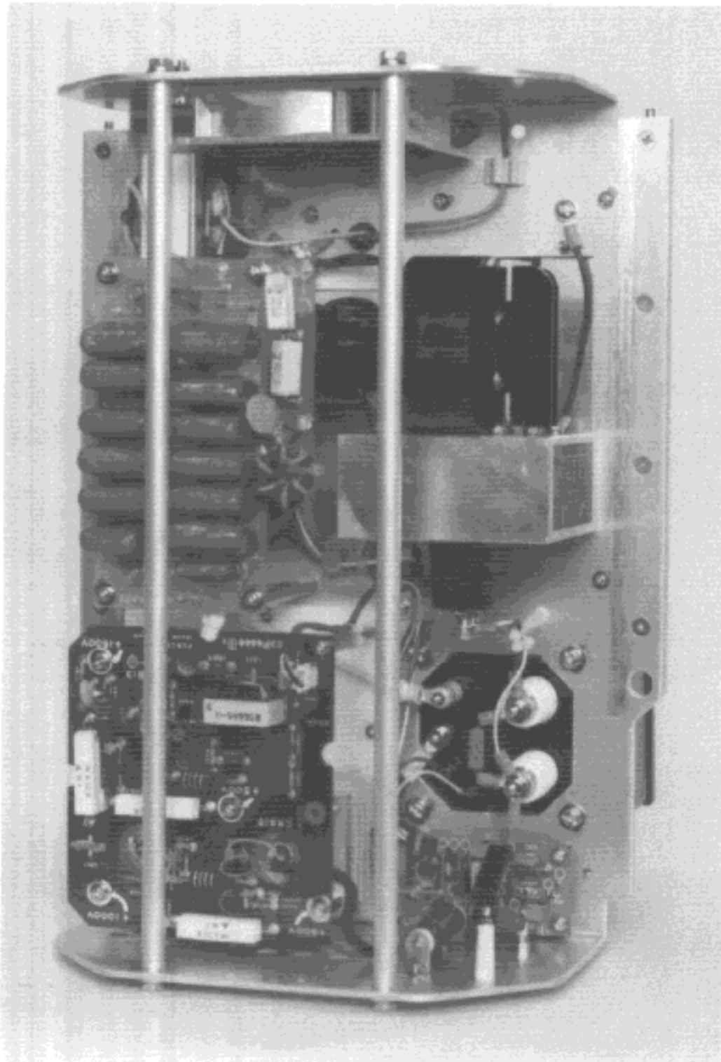
Photo 10.12 RF Module (Bottom cover removed)
