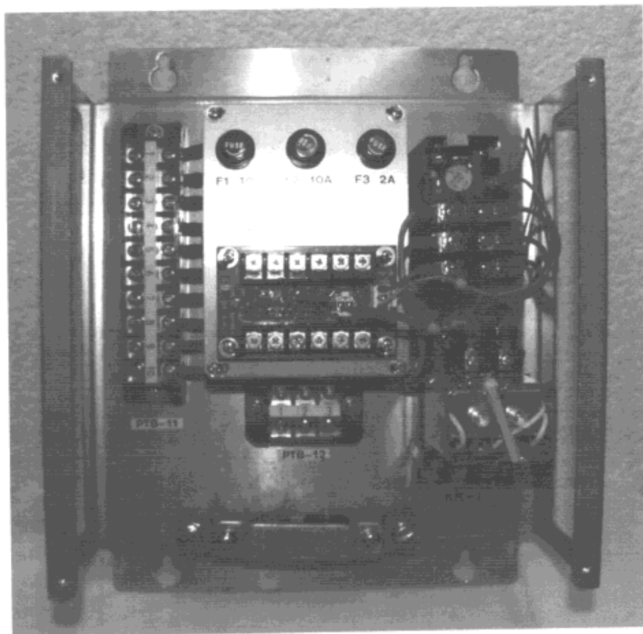
Photo 10.8 Power Supply Unit (PSU-004) Inside View (cover removed)
