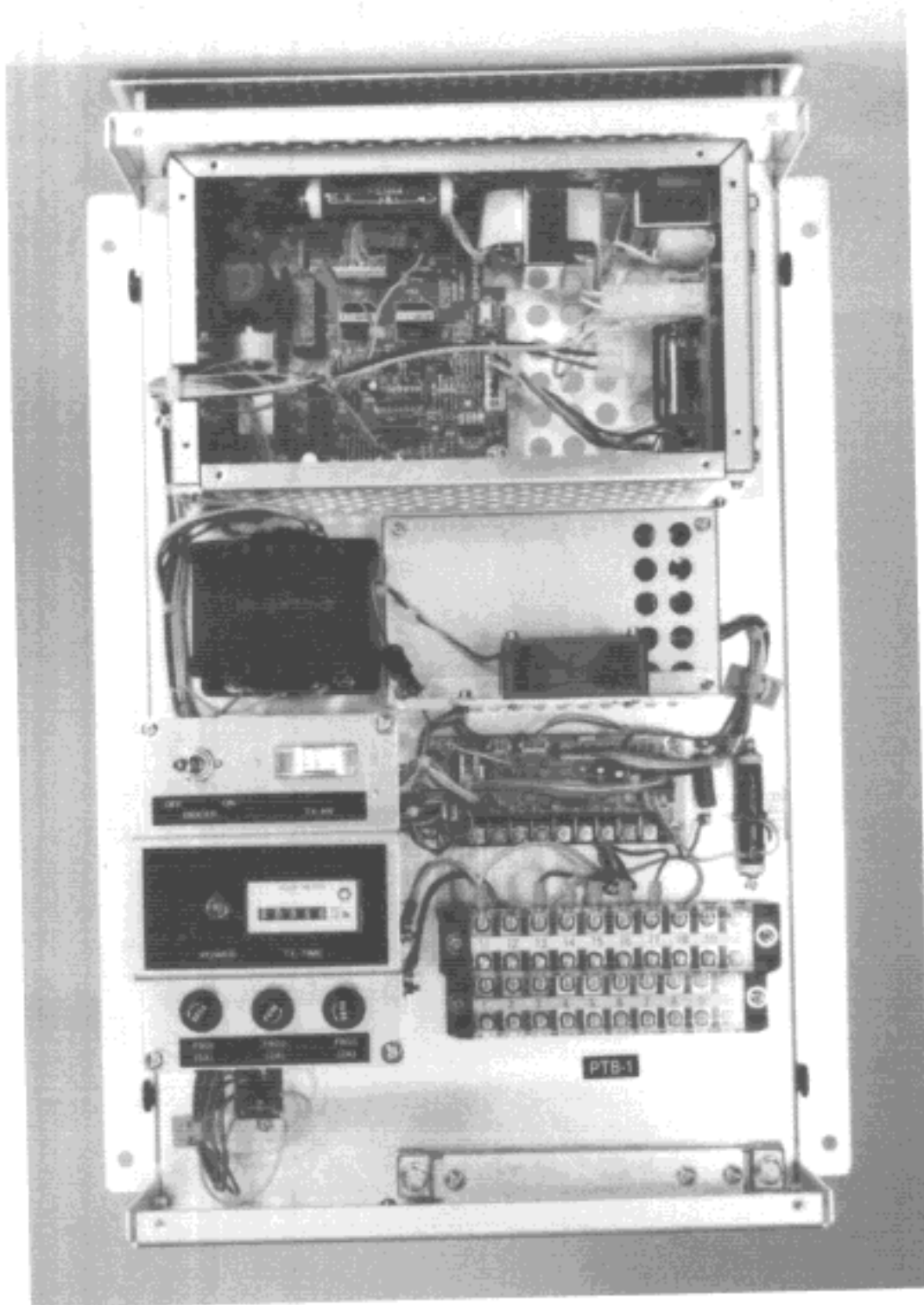
Photo 10.7 Power Supply Unit (PSU-001) Inside View (cover removed) (showing TX-HV and Power supply modules, Power Transformer and Terminal boards)
