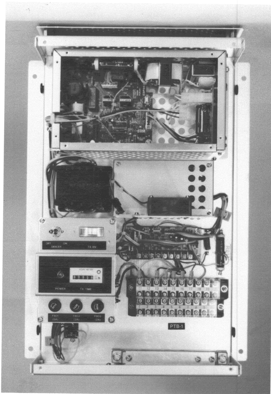
Photo 10.6 Power Supply Unit (PSU-002) Inside View (cover removed) (showing TX-HV and Power supply modules, Power Transformer and Terminal boards)
