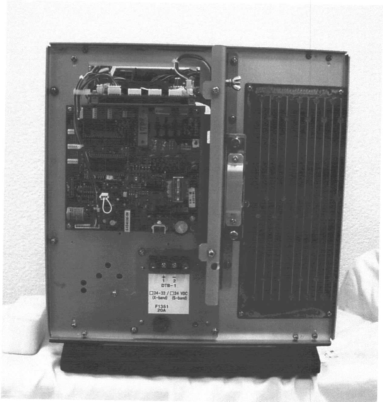
Photo 10.5 Display Unit (RDP-120) Rear View (cover removed) (showing GYRO CONVERTER (64P1106, option) board)
