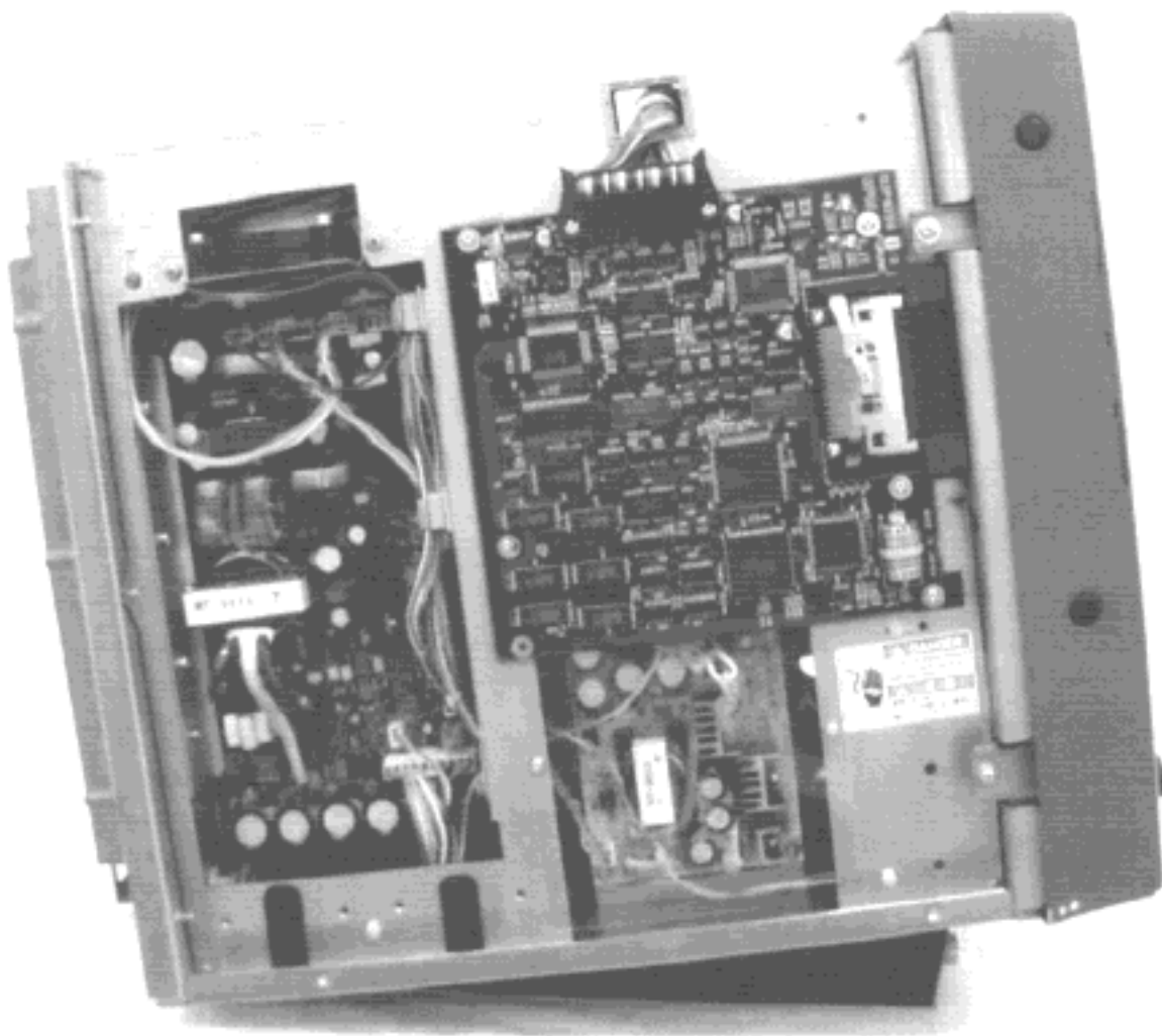
Photo 10.4 Display Unit (RDP-119) Left Side View (cover removed)
