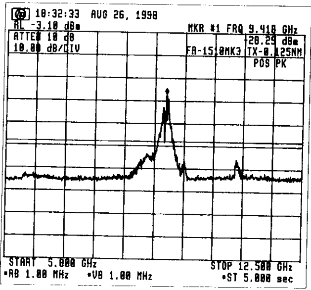
Fig. 1.2 With Filter No.1
