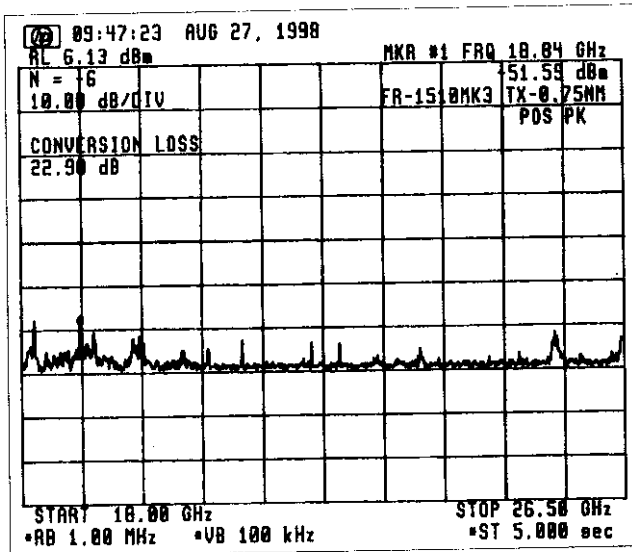
Fig. 3.4 With Filter No. 2
