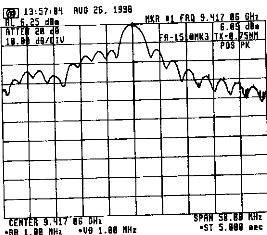
Fig. 4.4.3 For Middle 1 Pulse (0.75 nm Range)
