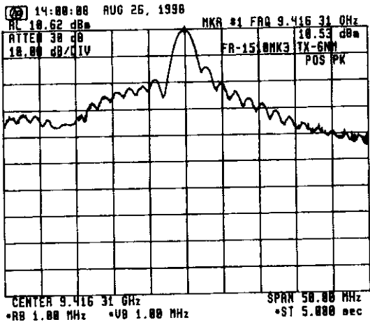
Fig. 4.4.4 For Middle 2 Pulse (6 nm Range)
