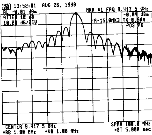
Fig. 4.4.2 For Short 2 Pulse (0.5 nm Range)
