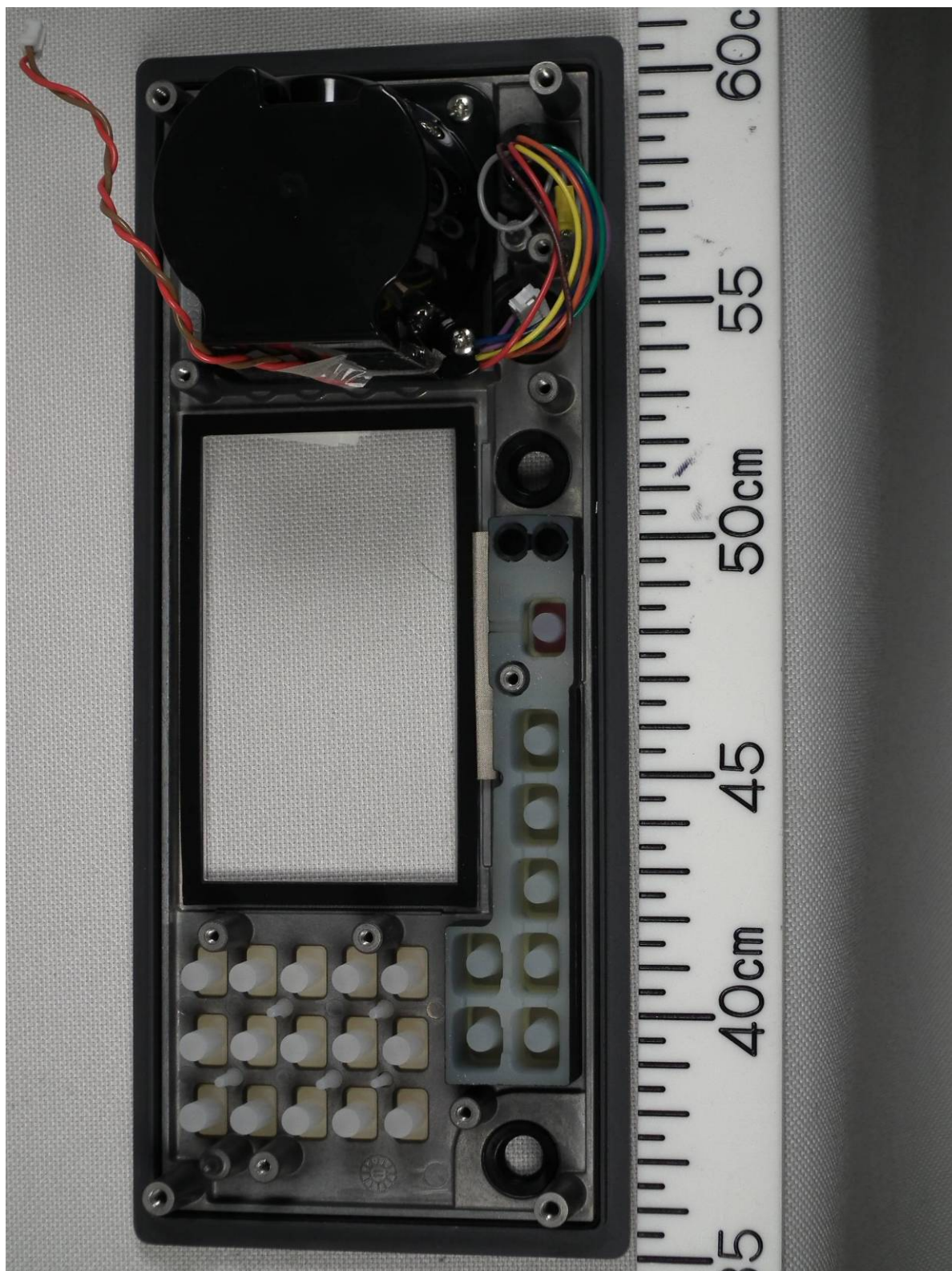
1.17 Back of Front Panel (with PANEL Board removed)
