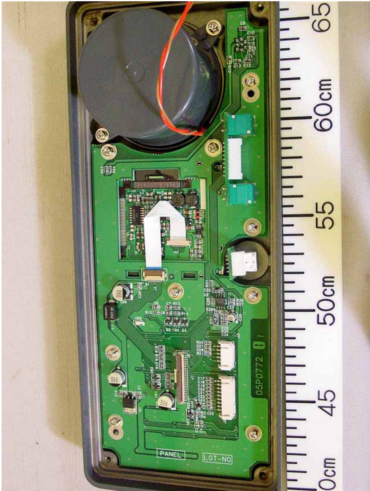
1.16 Panel Inside View (showing PANEL Board 05P0772 Rear side)
