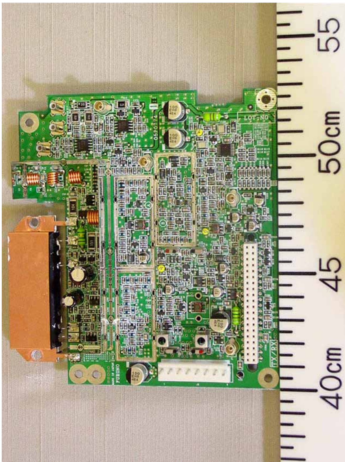
1.5 TX / RX Board 05P0774 Front side
