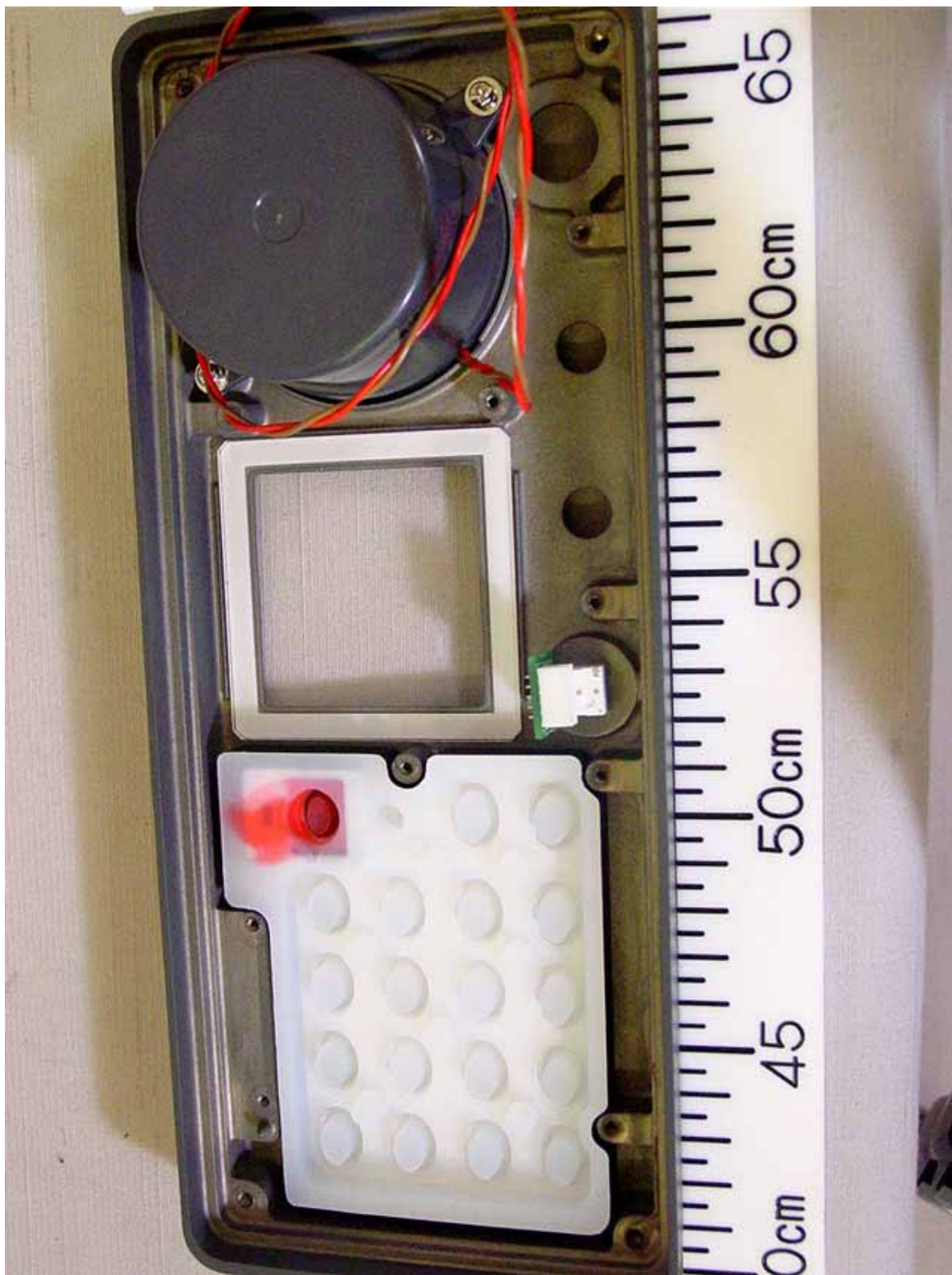
1.17 Panel Inside View (with PANEL Board removed, showing Back of Front Panel)
