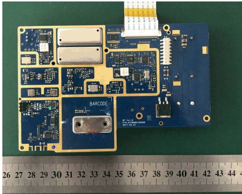
EUT- Main Board 1 Top View
