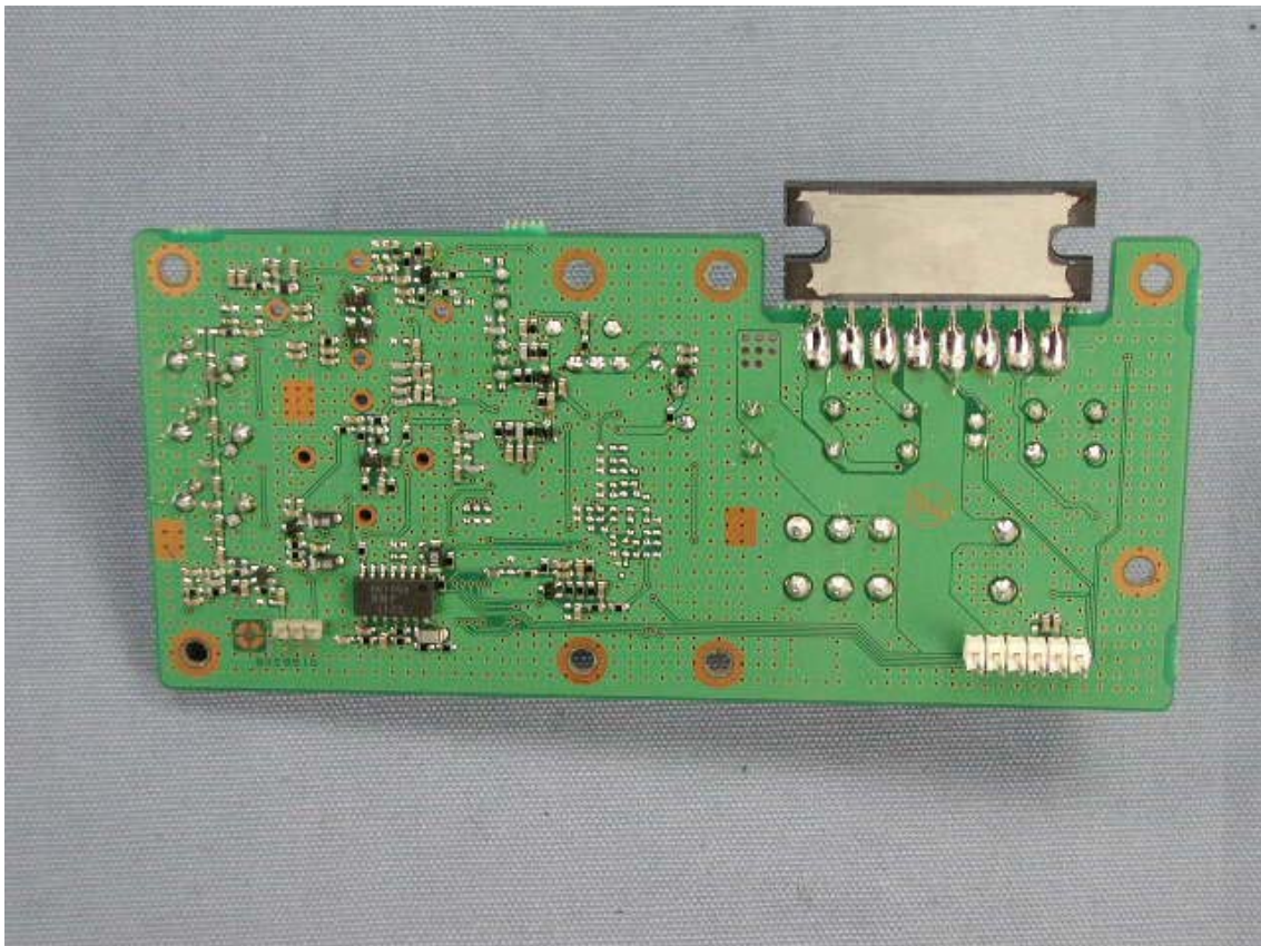
Side-B of SUB-unit
