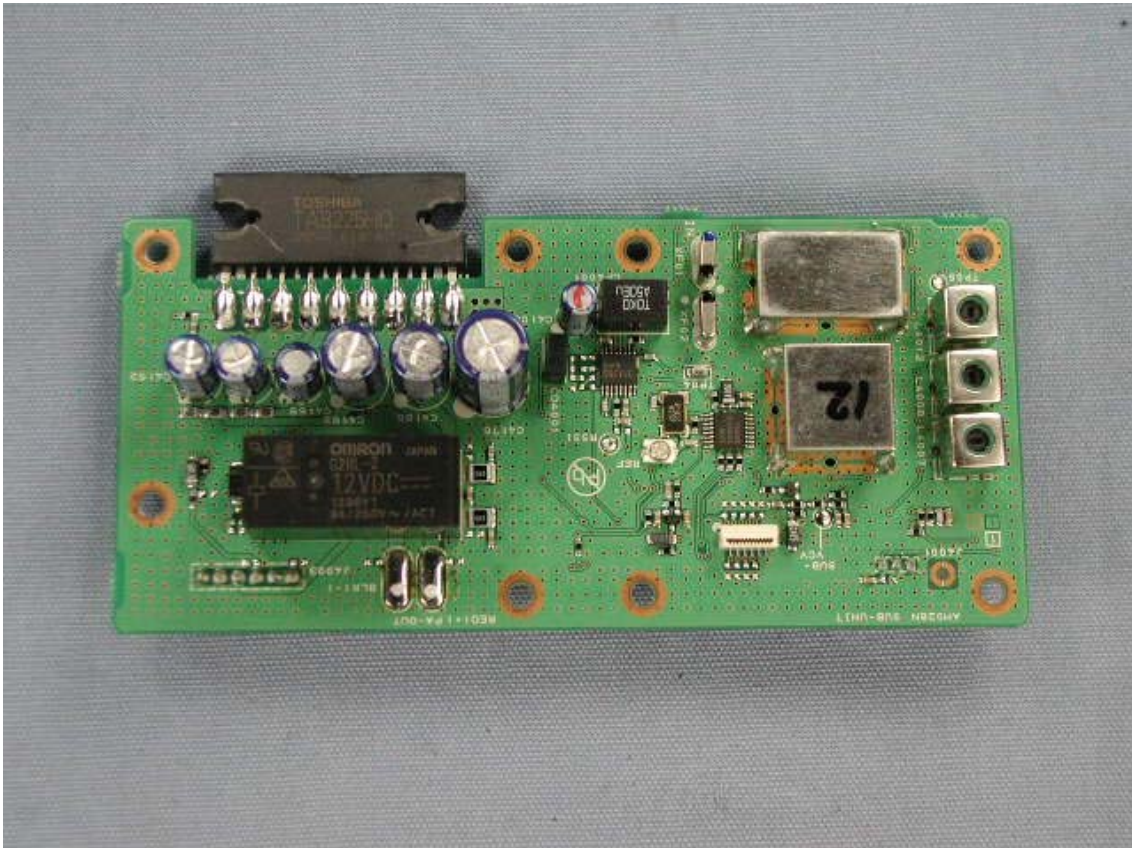
Side-A of SUB-UNIT with shield cases
