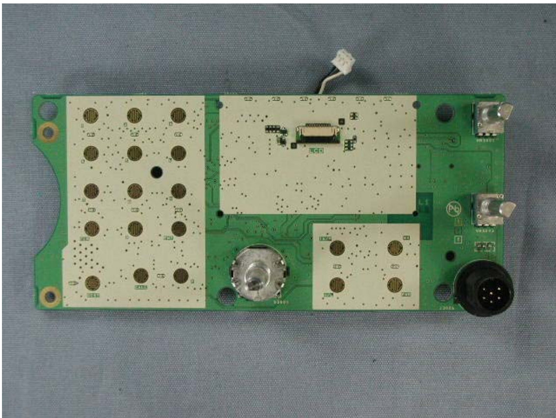
Side-A of CNTL-2-UNIT without LCD
