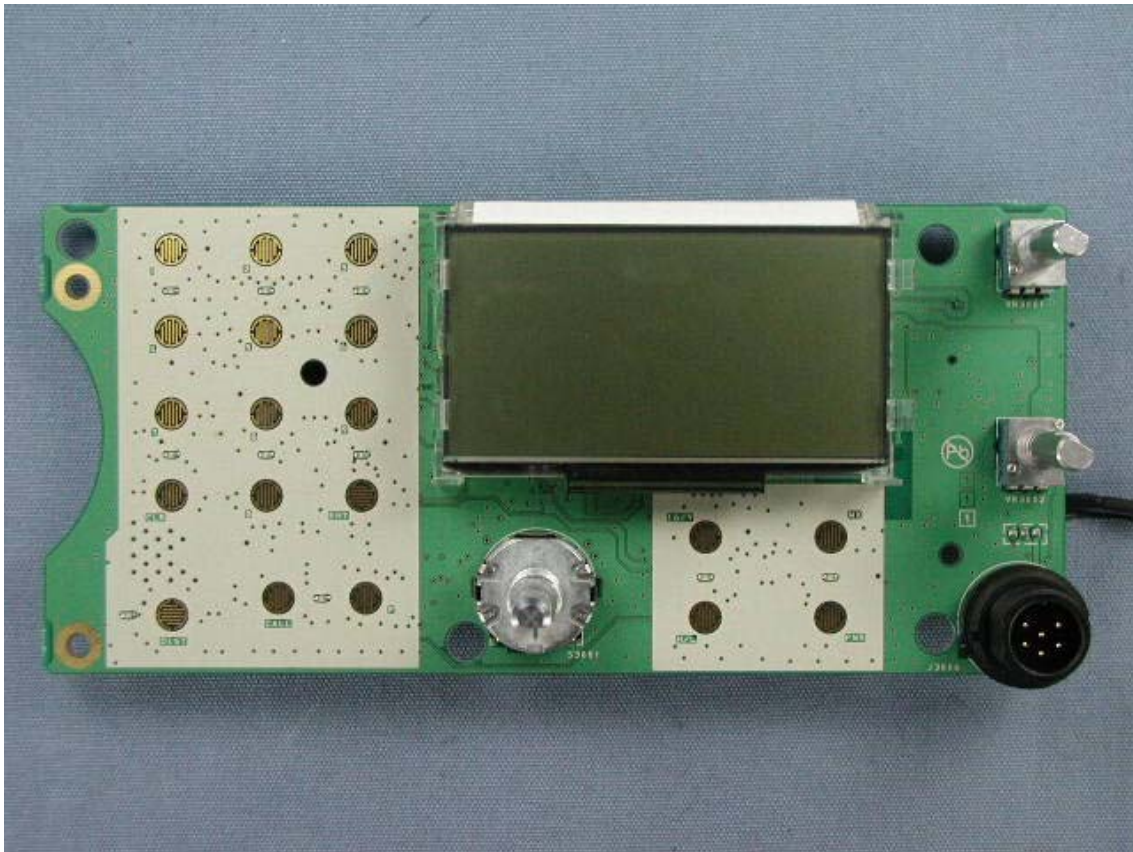
Side-A of CNTL-2-UNIT with LCD
