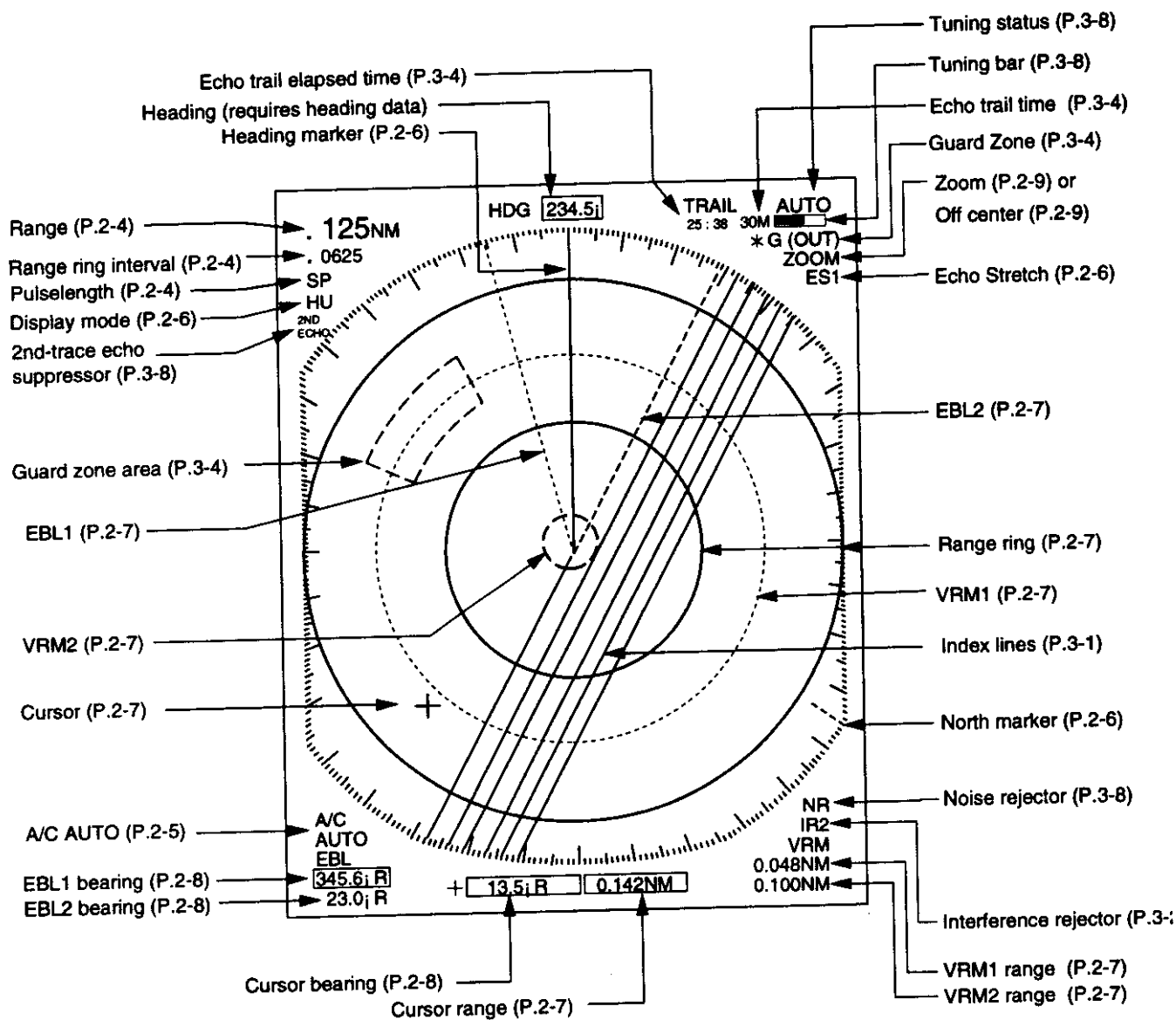
Figure 2-2 Display indications
