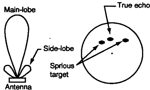
Figure 4-2 Side-lobe echoes
