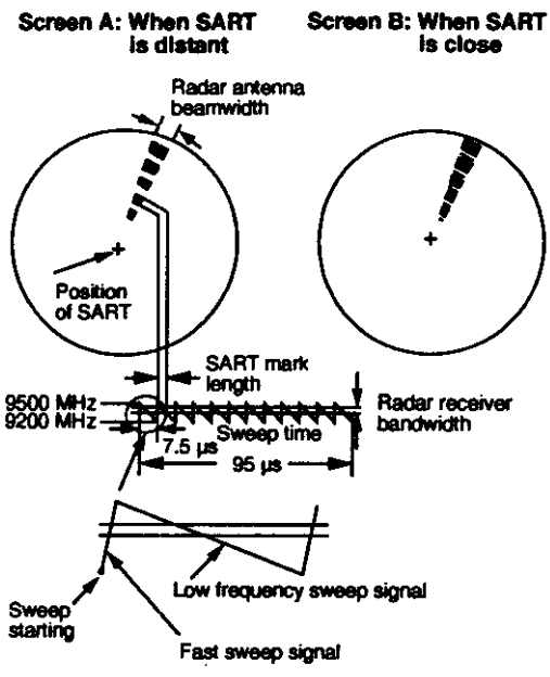
Figure 4-5 SART display
