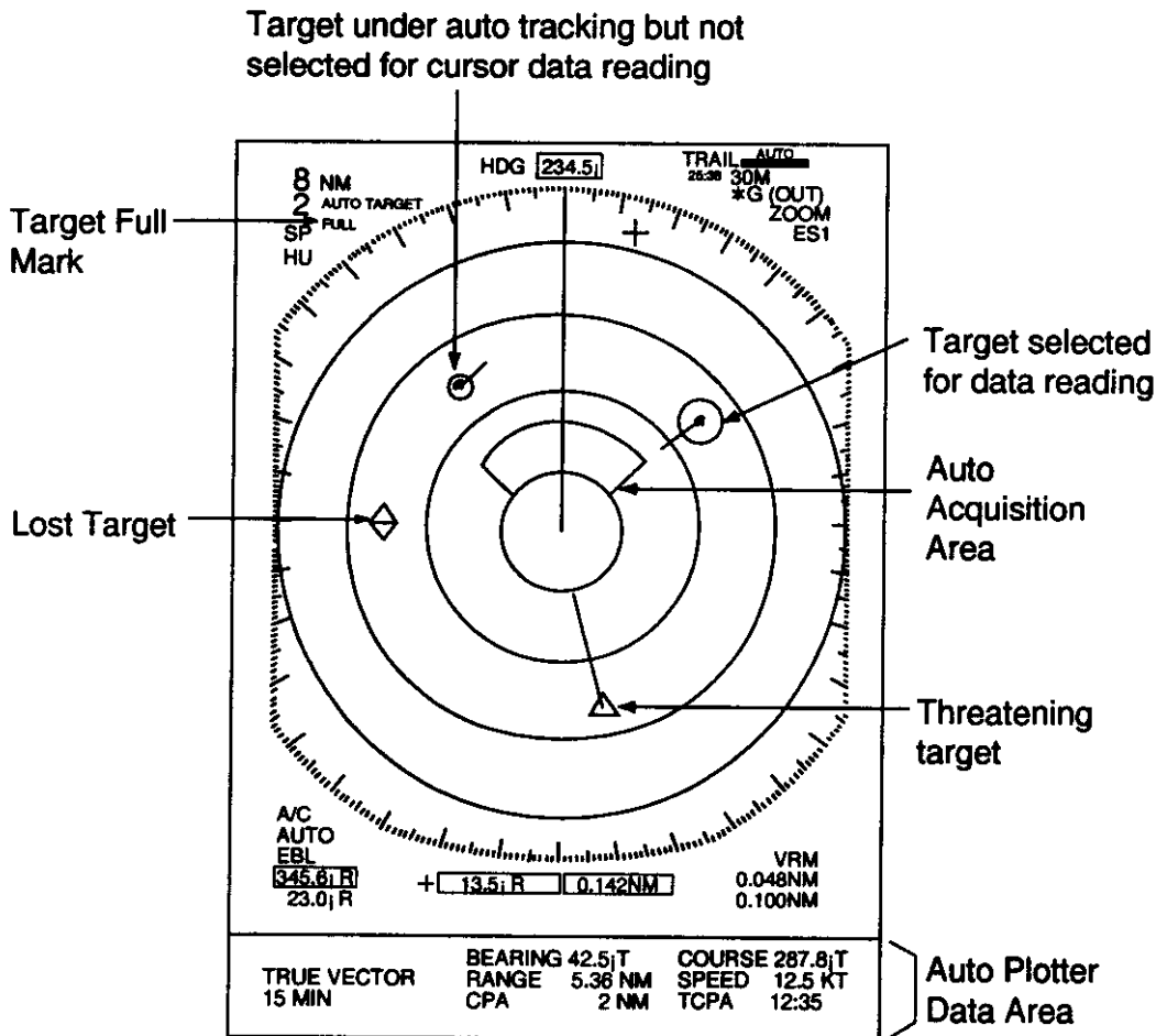
Figure 6-2 ARPA display
