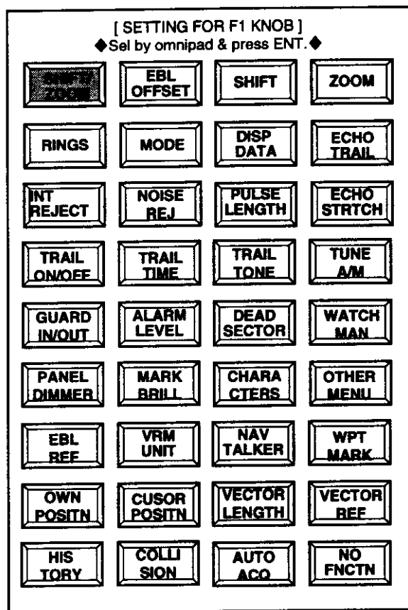
Figure 3-11 Function menu
