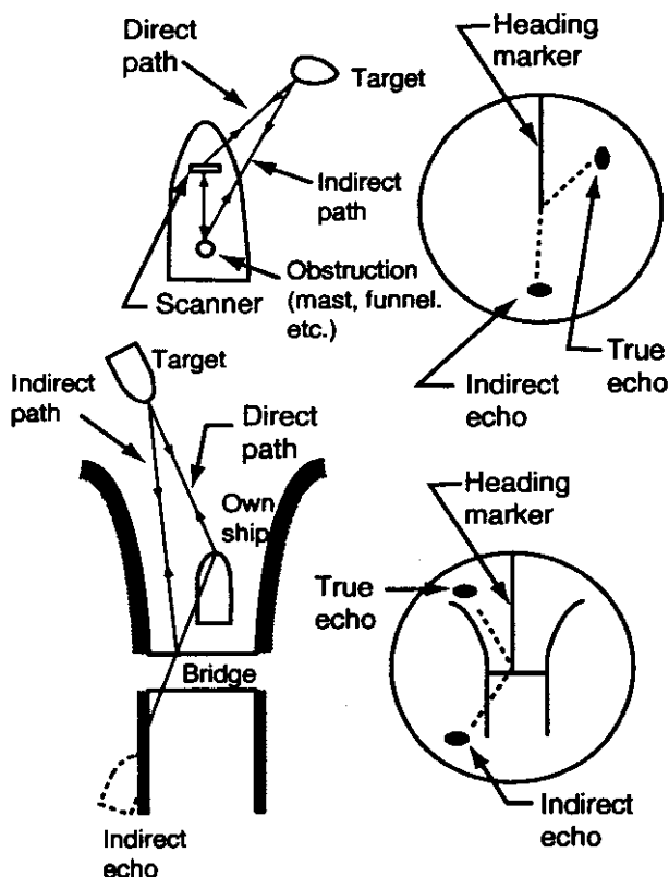
Figure 4-3 Indirect echoes
