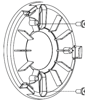
(Mounting Bracket)
