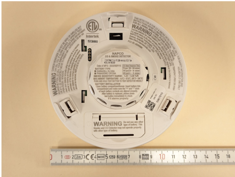
Bottom with Mounting Plate removed
