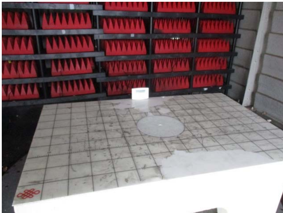
Spurious Radiated Emissions, EUT Configuration
