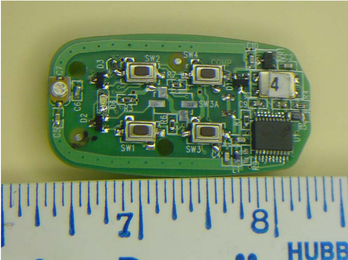
Top of PCB, antenna is integral and can be seen as the etch around the edge of the PCB
