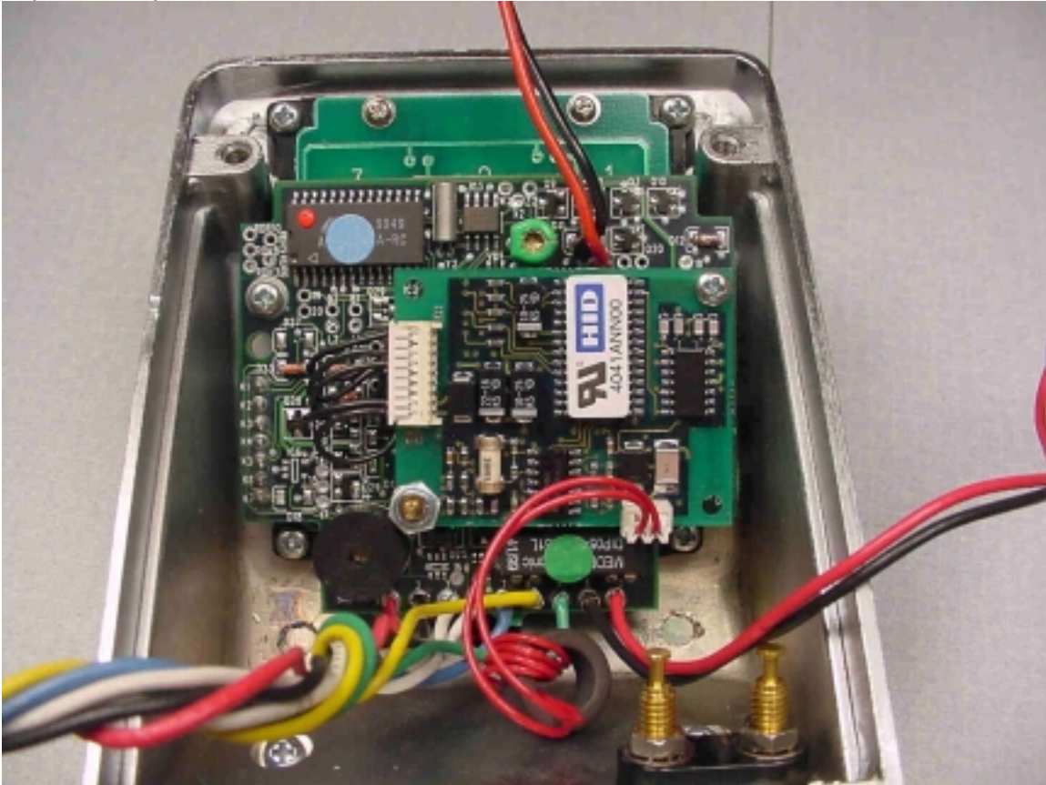
Rear of Electronics Housing with cover removed
