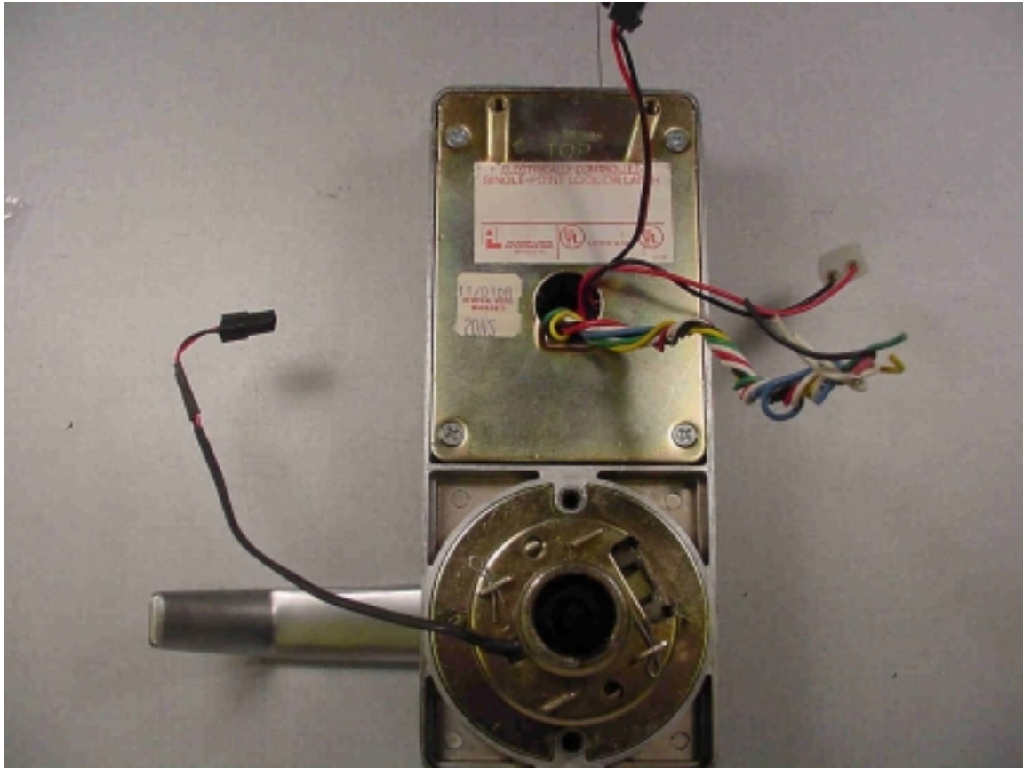
Rear of Electronic control housing when removed from door
