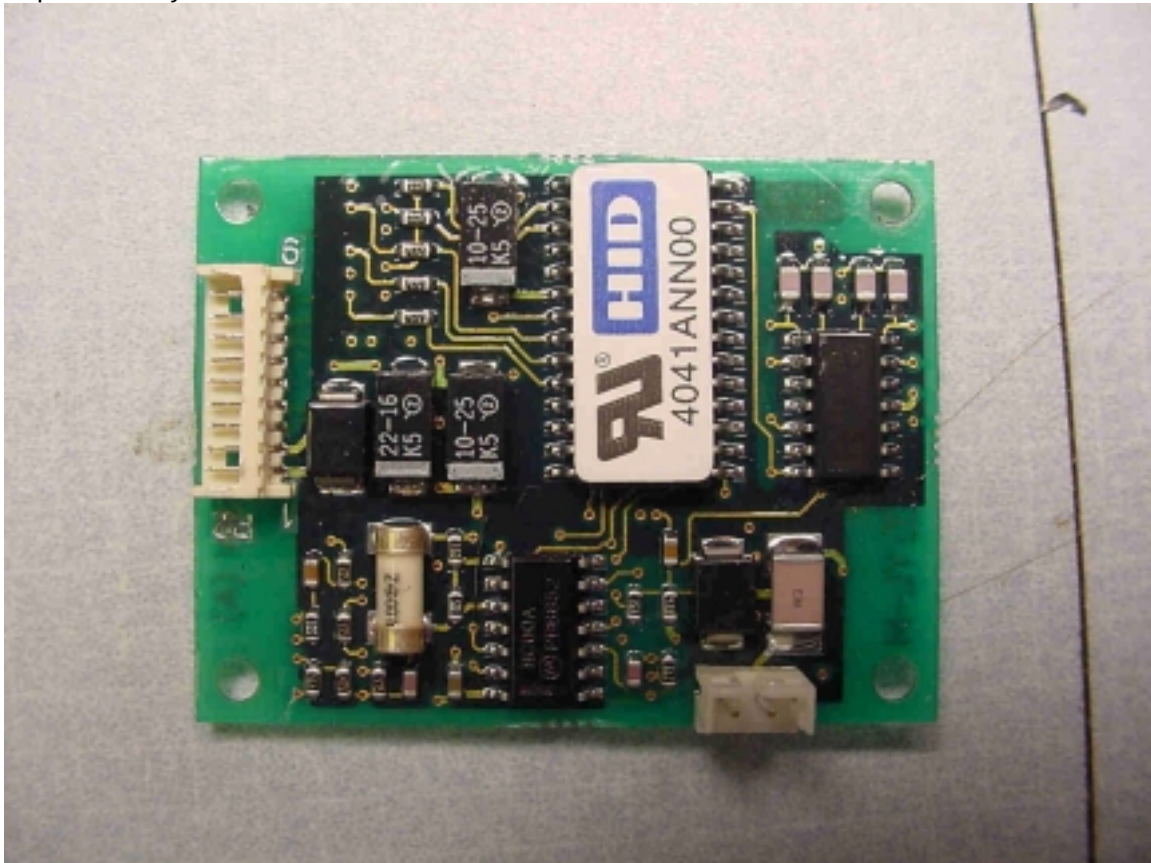
Front of Tx PCB
