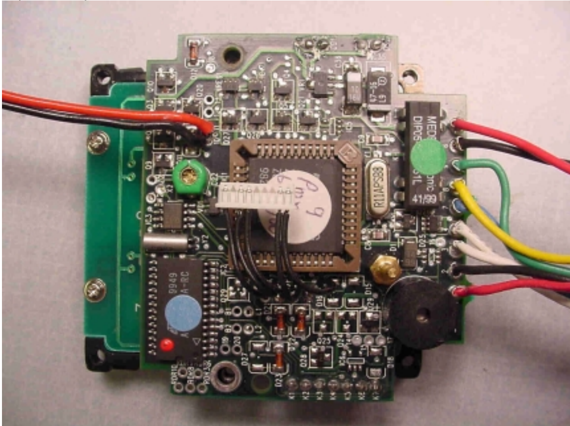
Front of the Main Circuit Board
