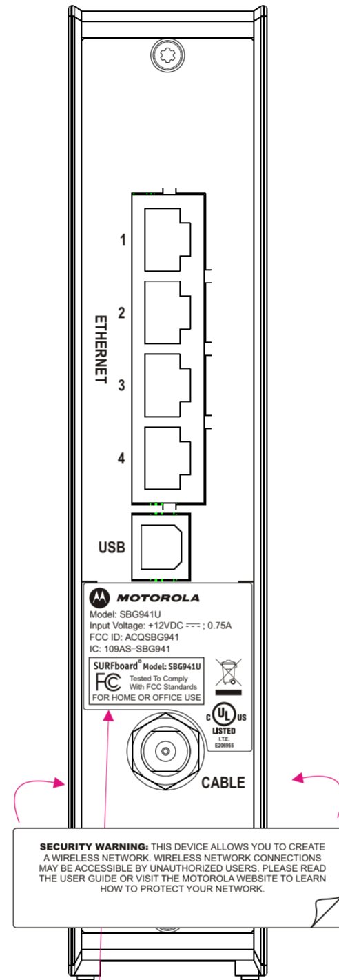
Model: SBG941U Shown Regulatory label & Rear Label for Vertical Installation
