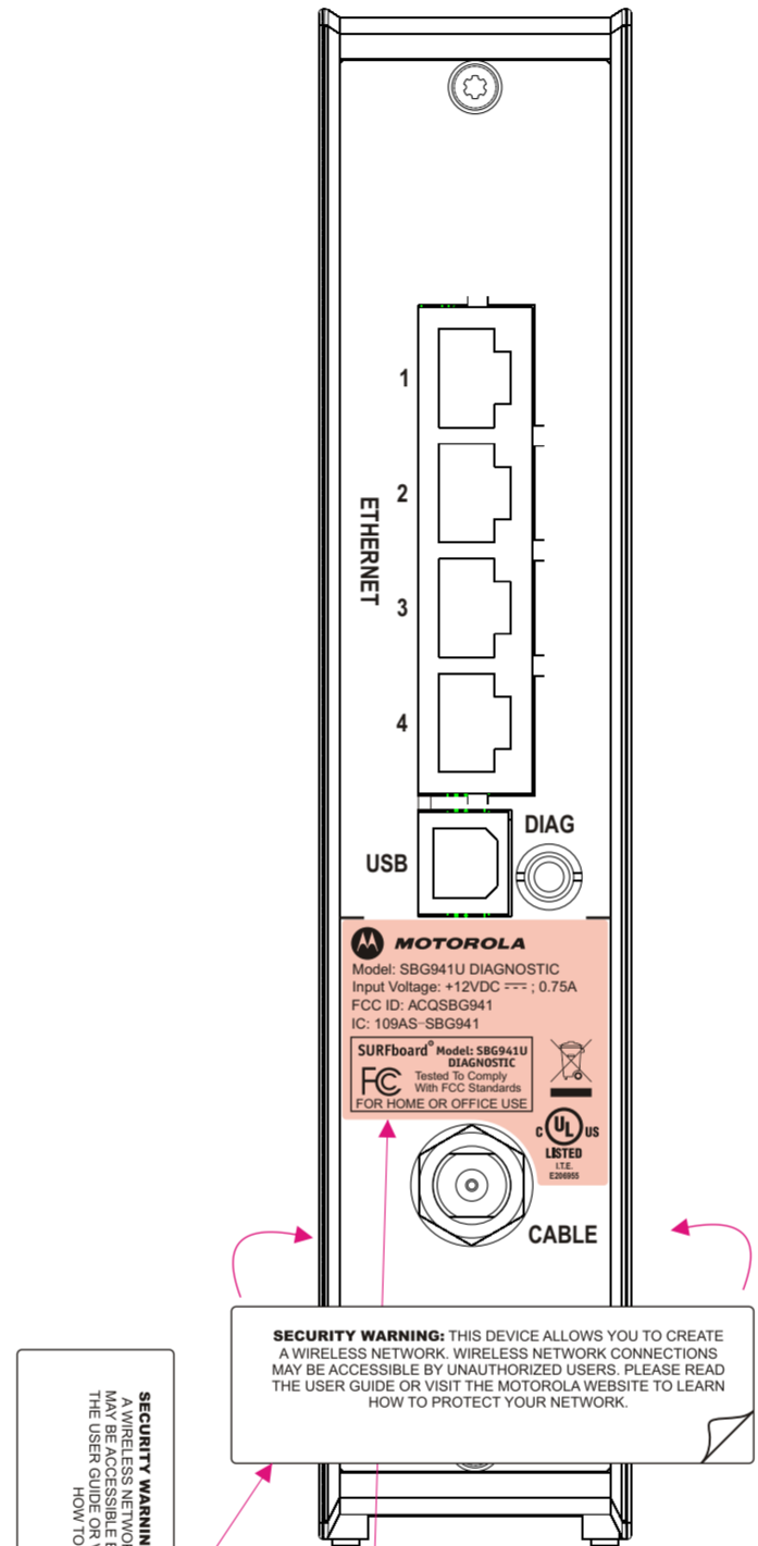
Model: SBG941U Diagnostic Shown Regulatory label & Rear Label for Vertical Installation
