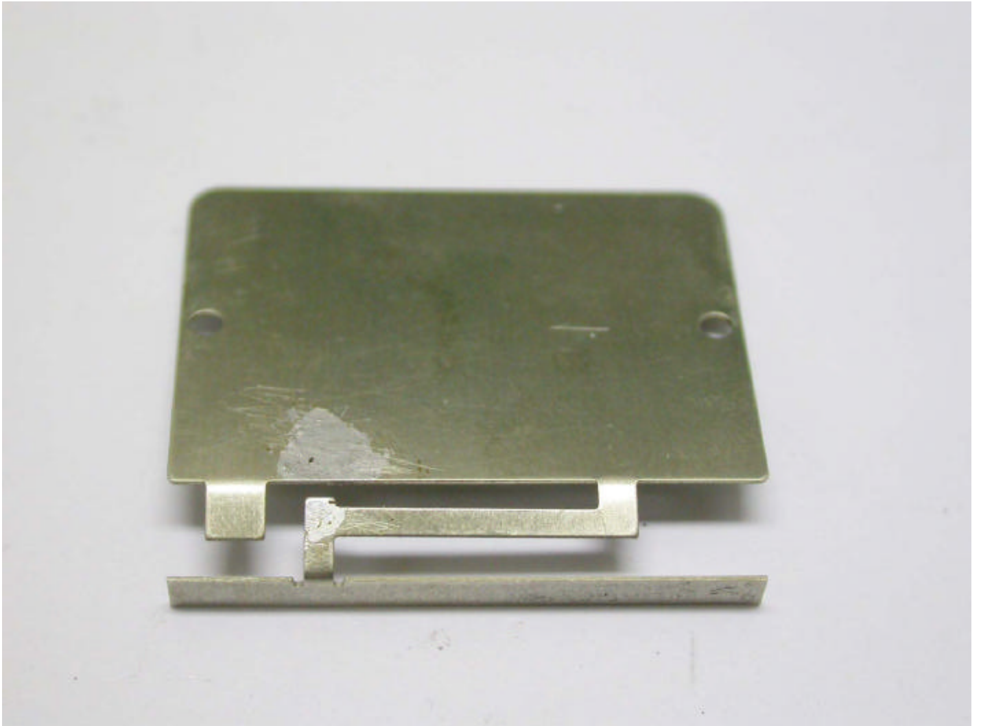
Antenna type 2: Intenna PIFA antenna
