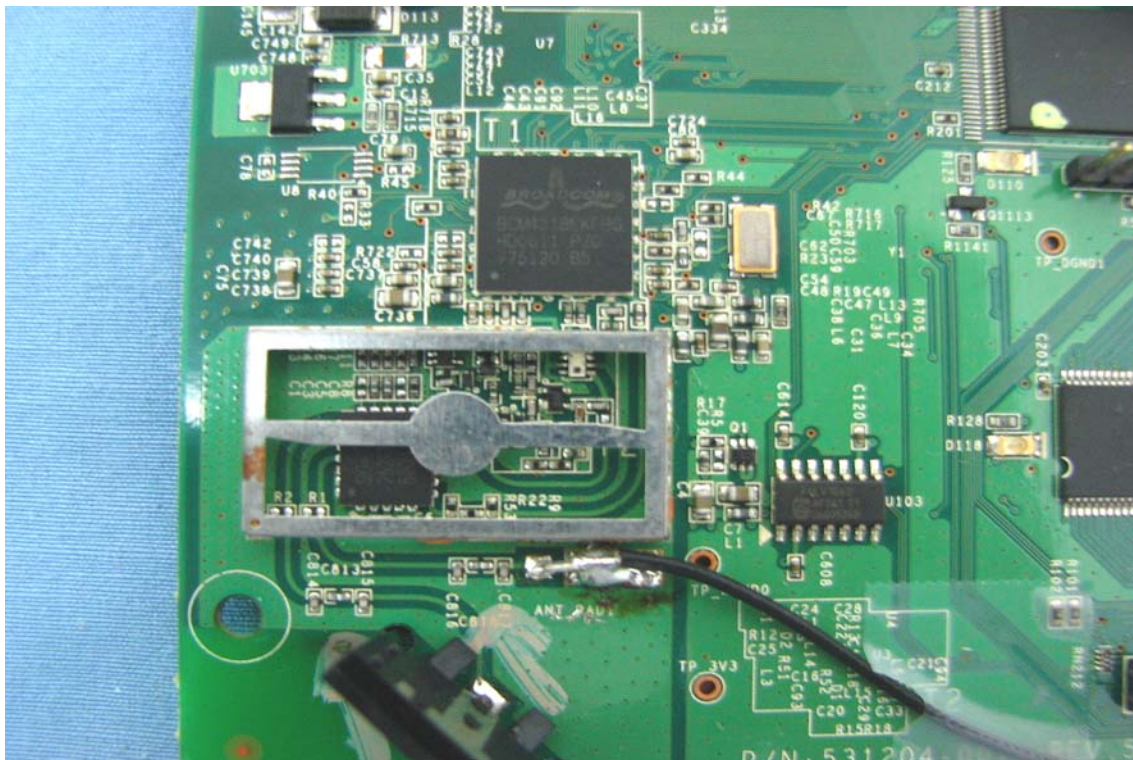
T-Stub Antenna
