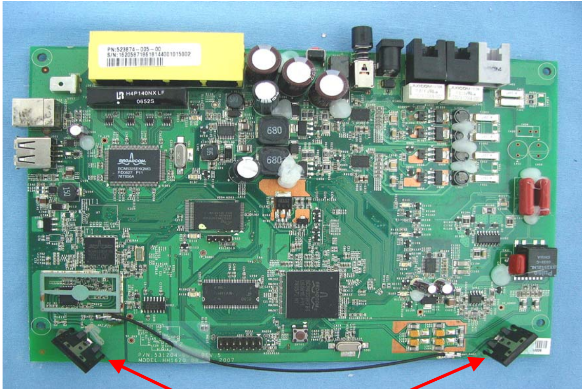
T-Stub Antenna
