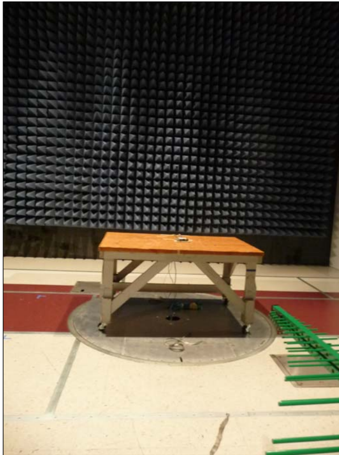
Photograph 2. Radiated Emissions Test Setup, Antenna
