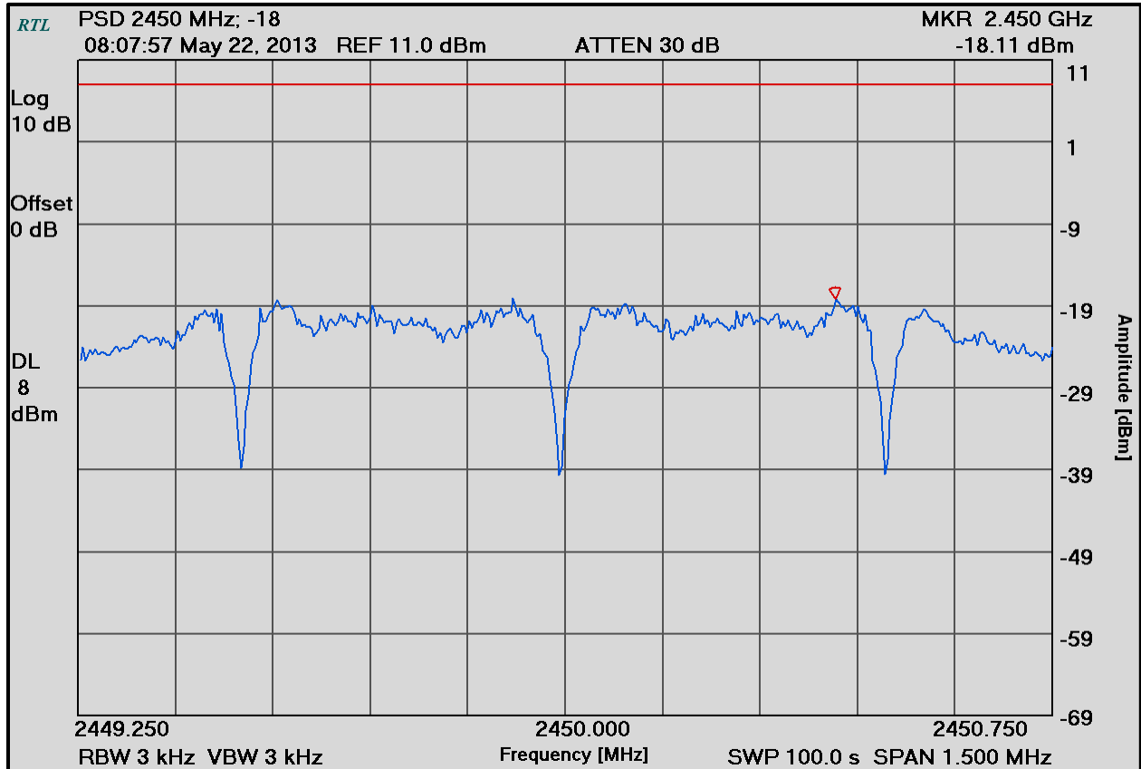
Plot 8-2: Power Spectral Density (2450 MHz)
