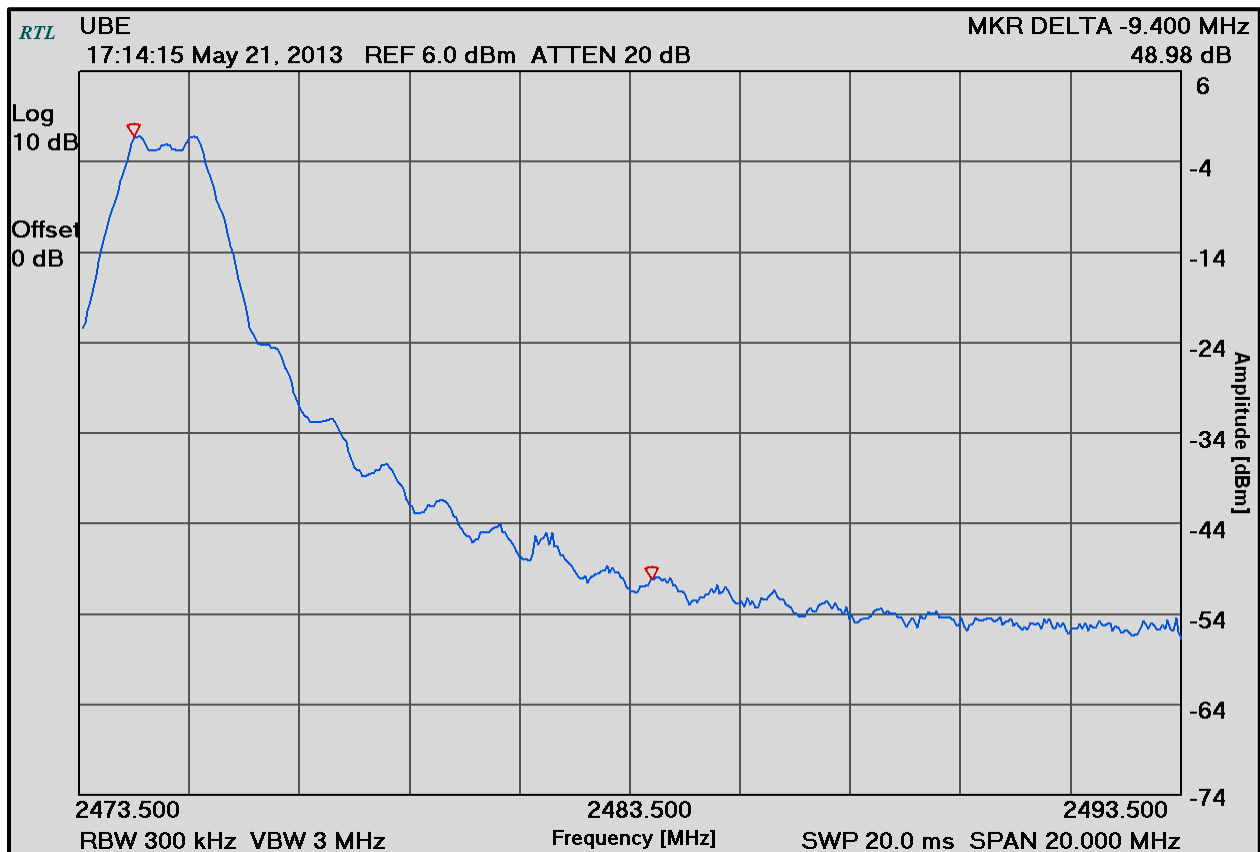
Plot 5-2: Upper Band Edge (2475 MHz)
