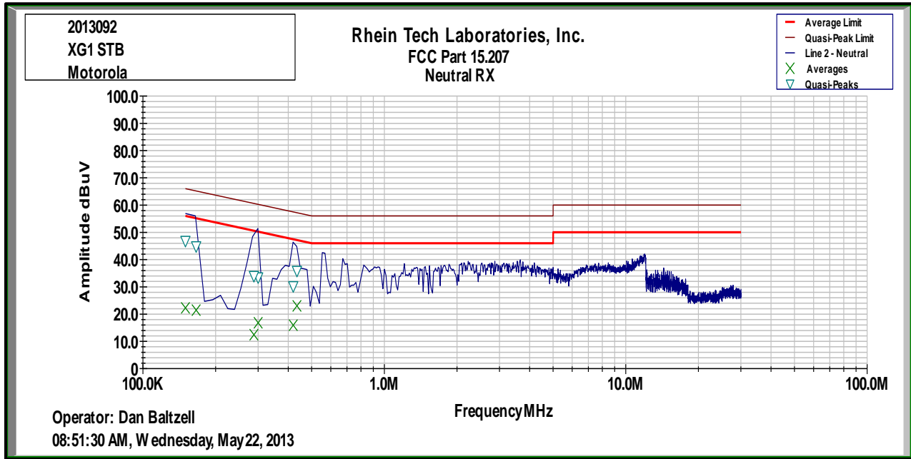
Plot 9-1: Conducted Emissions Test Data – Neutral - RX Mode
