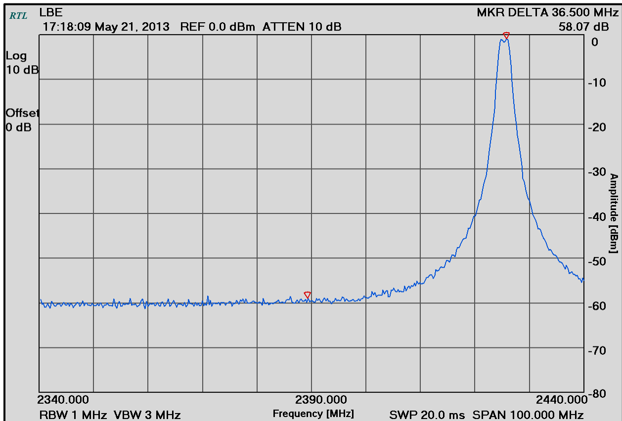
Plot 5-1: Lower Band Edge (2425 MHz)
