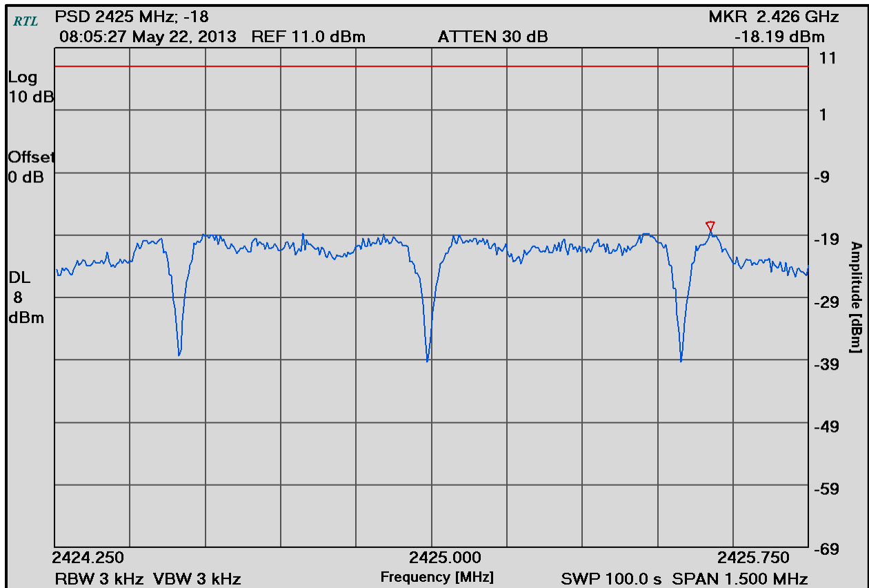
Plot 8-1: Power Spectral Density (2425 MHz)
