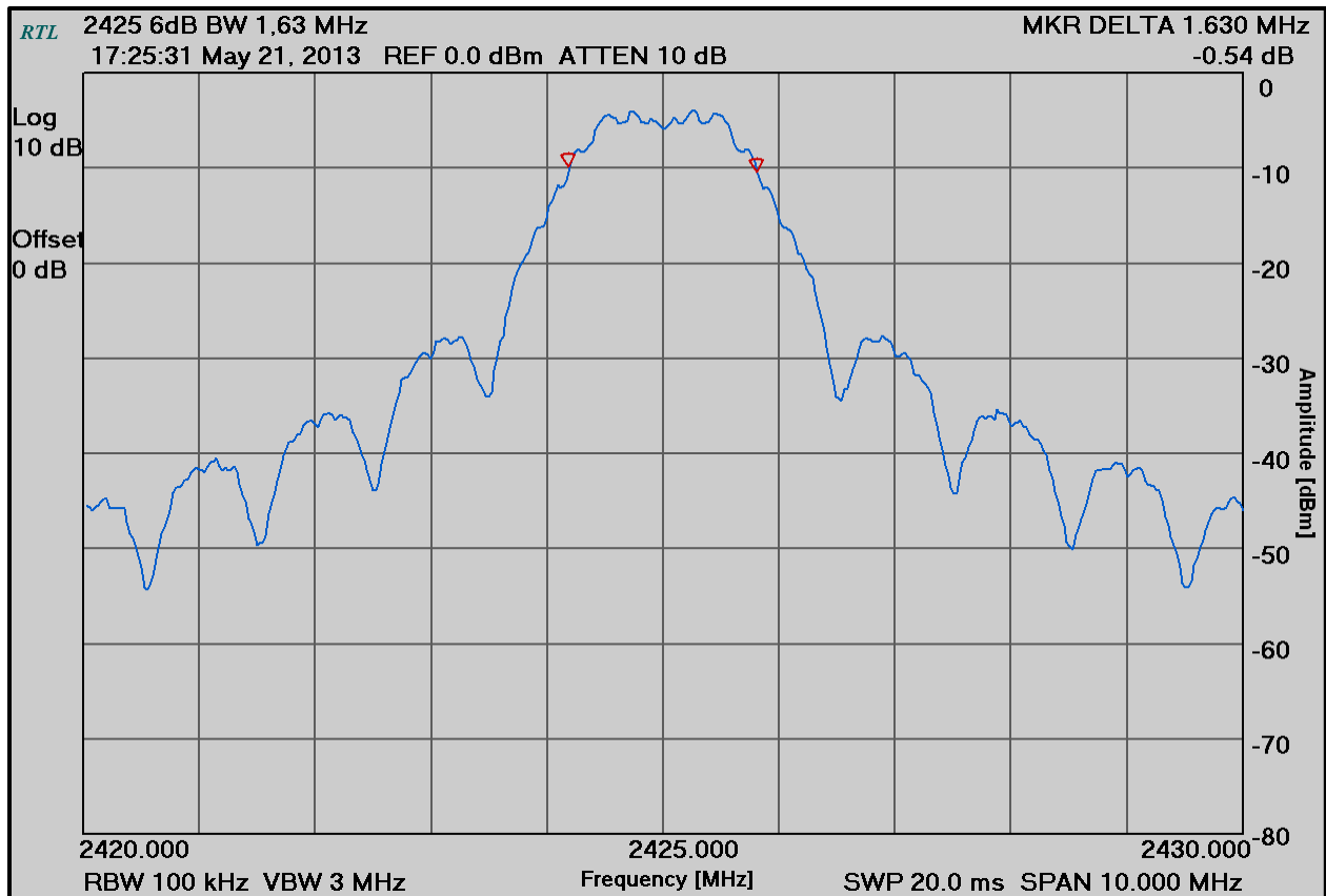
Plot 7-1: 6 dB Bandwidth (2425 MHz)
