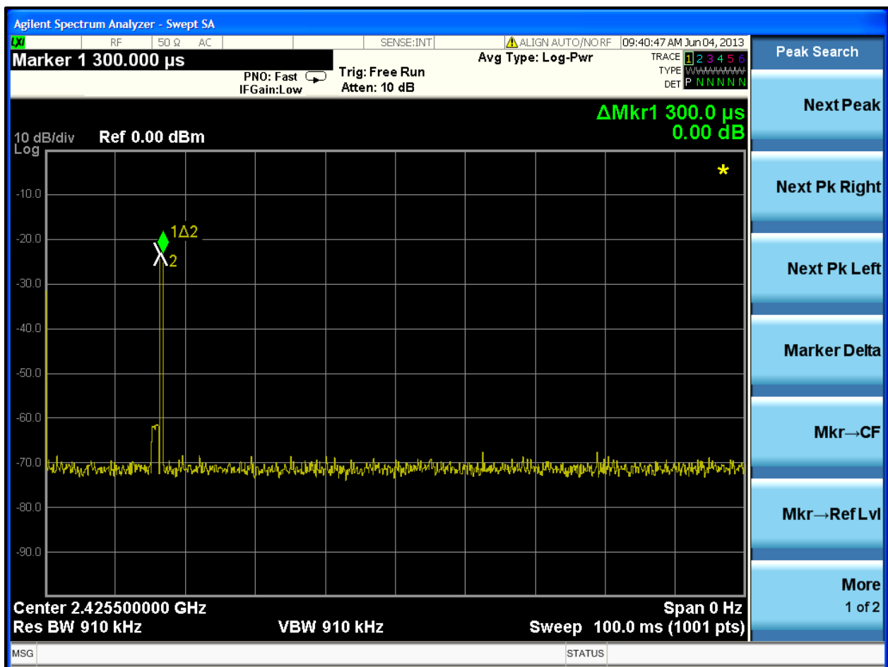
Plot 4-1: Duty Cycle in 100ms
