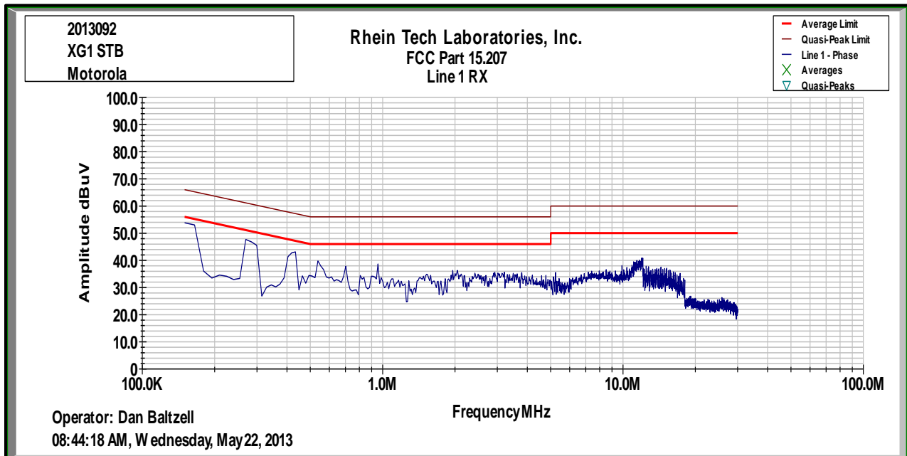
Plot 9-2: Conducted Emissions Test Data – Hot – RX Mode
