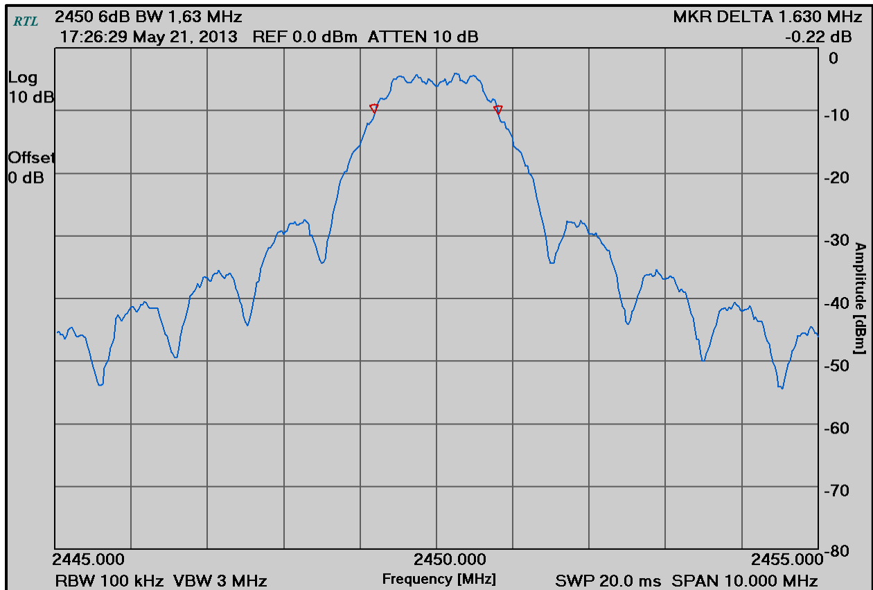
Plot 7-2: 6 dB Bandwidth (2450 MHz)
