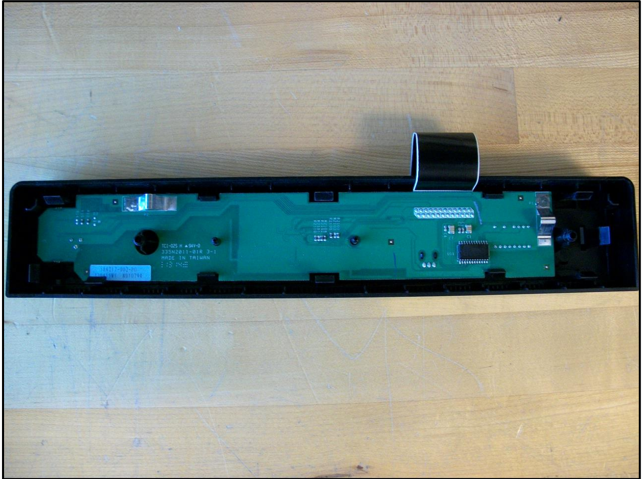
Photograph 13: Bezel PWB Rear
