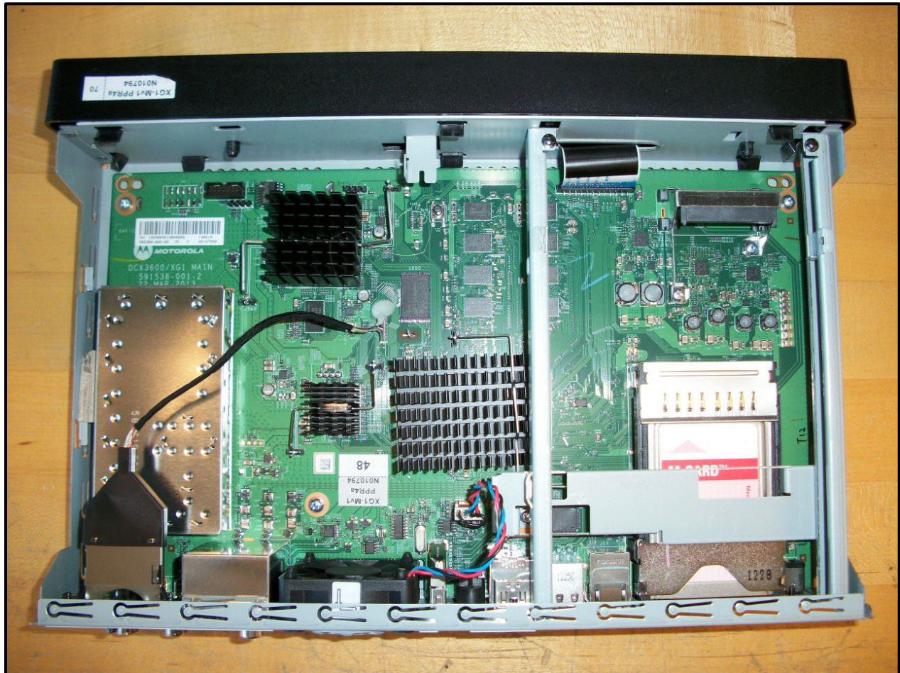
Photograph 11: HDD Removed
