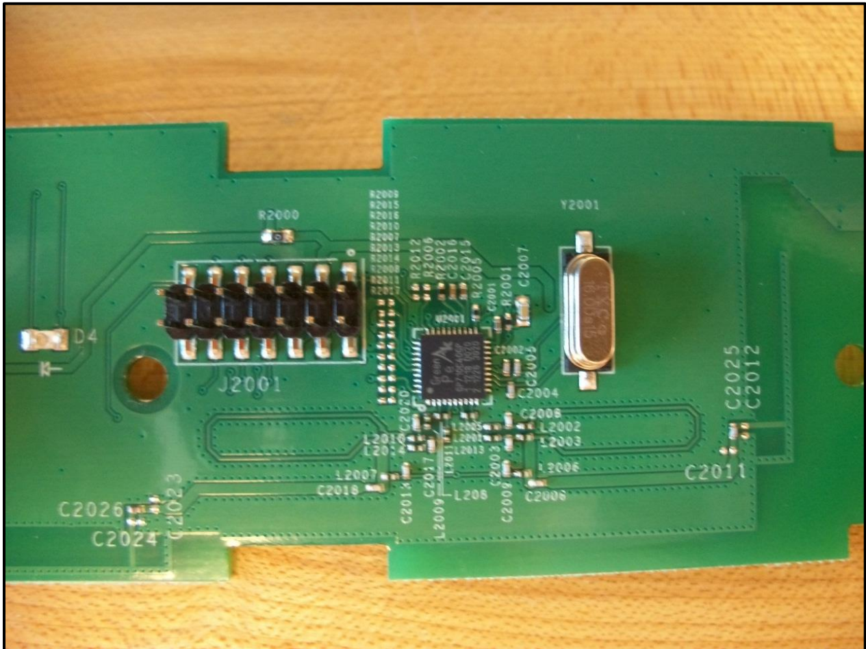
Photograph 14: RF4CE Circuit Antenna
