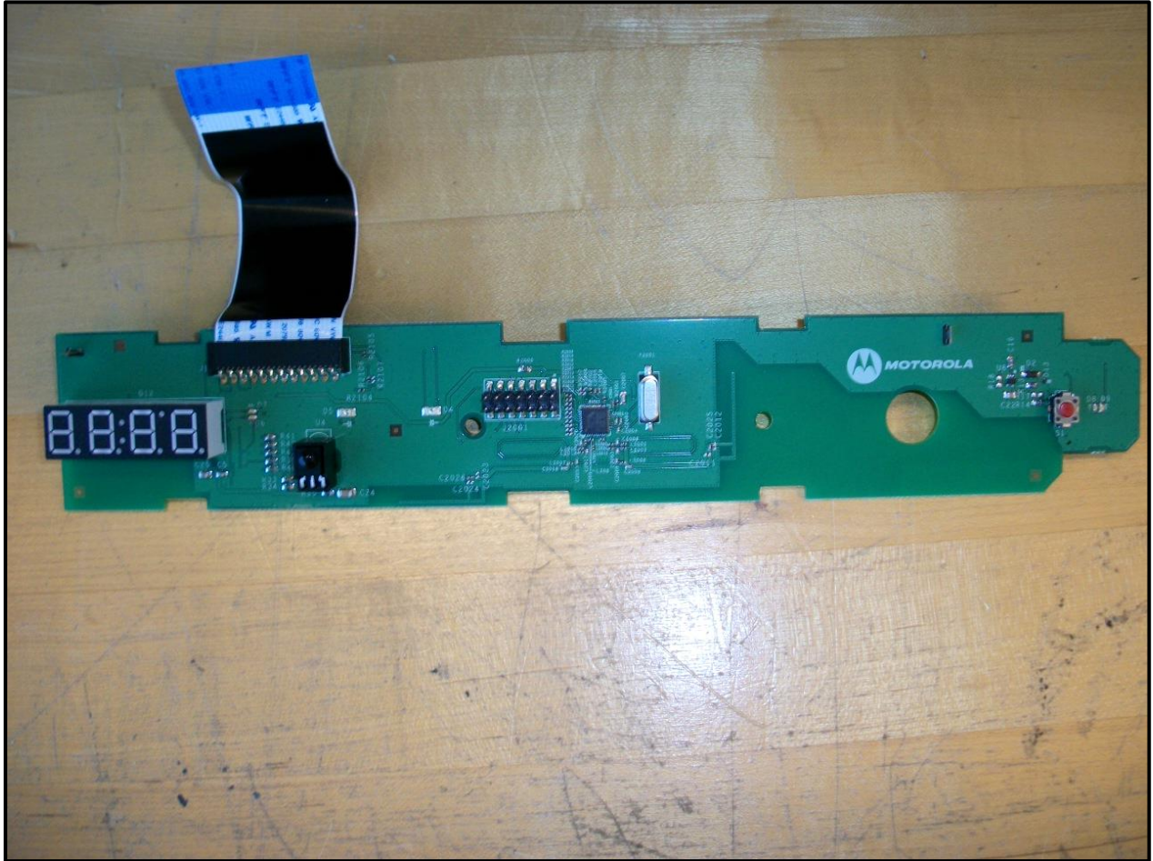
Photograph 12: Bezel PWB Front
