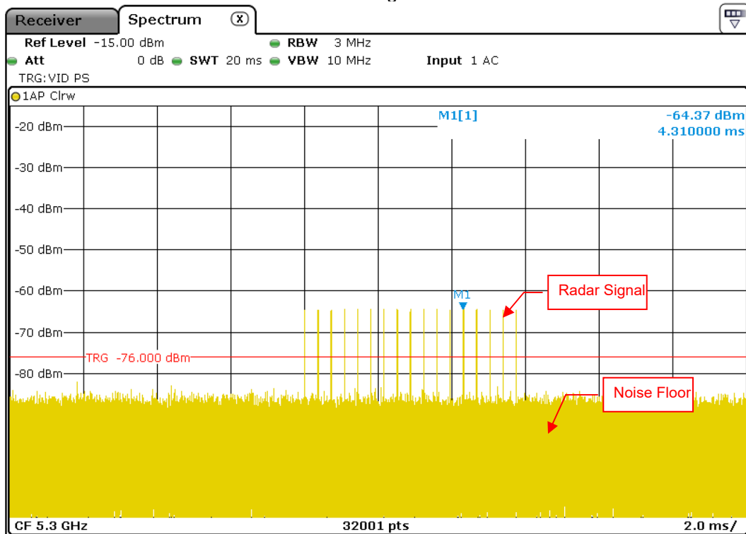
Radar Signal 3
