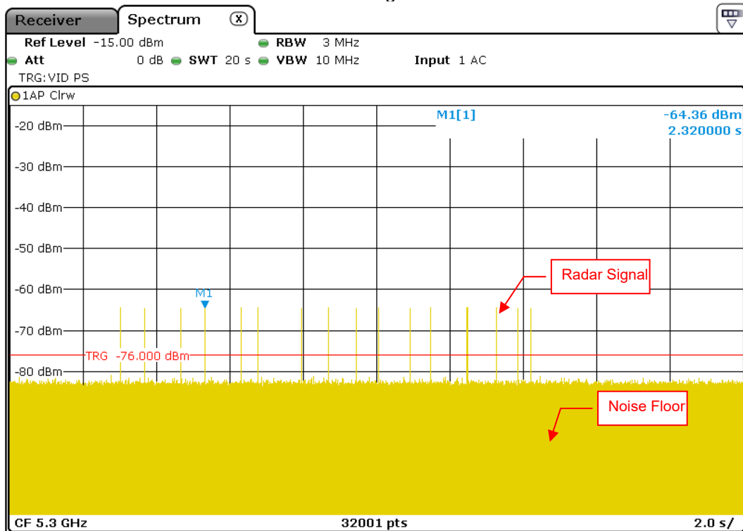
Radar Signal 5
