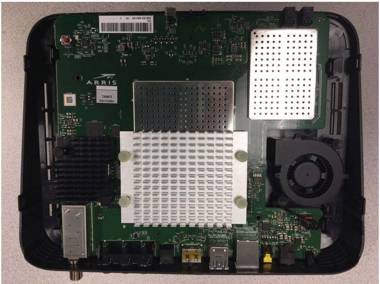
VMS4100 BOARD WITH SHIELDS
