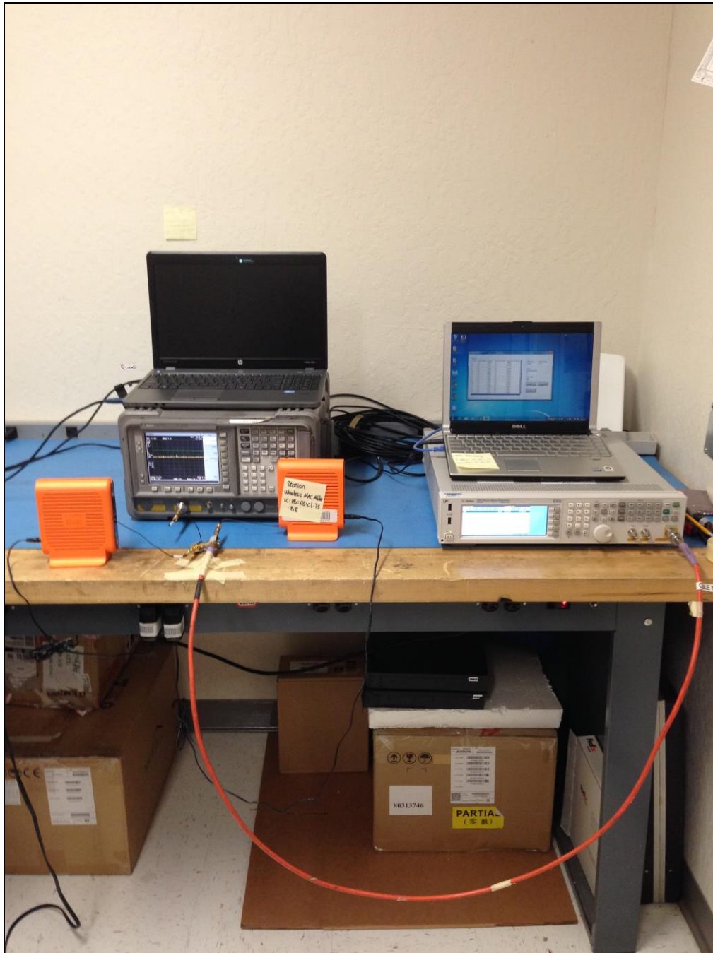
Photograph 2. DFS, Test Setup
