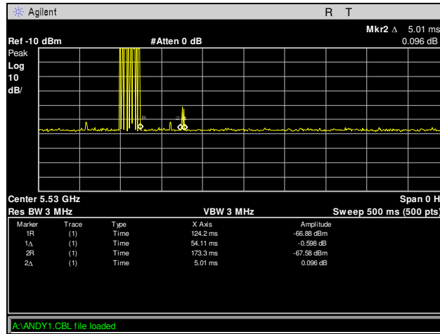
Plot 22. DFS Channel Closing Transmission, Time Aggregate, 80 MHz, Channel 106
