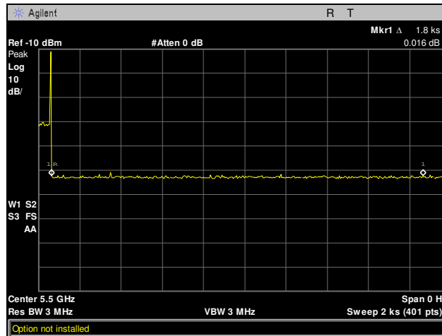
Plot 26. Non-Occupancy, 80 MHz, Channel 100
