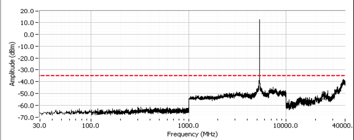
802.11 a, 5320 MHz, Chain 3
