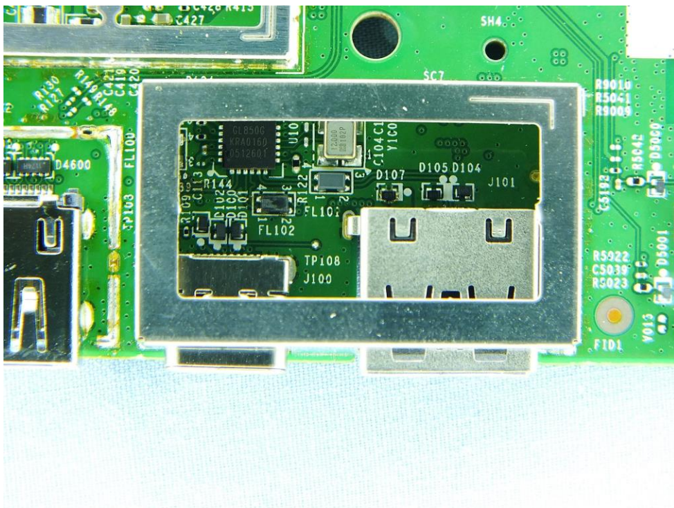
USB chip: GL850G
