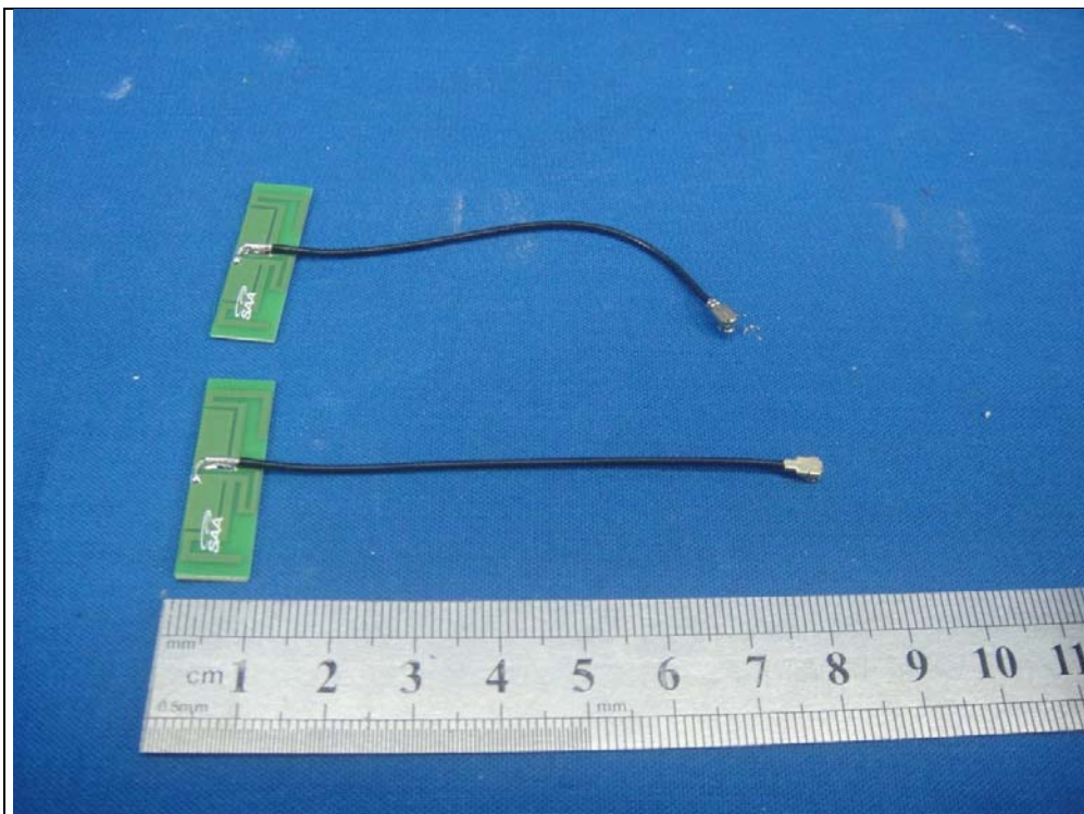
Antenna set 4(Model: RR7512-15-000-C / RR7513-15-000-C)
