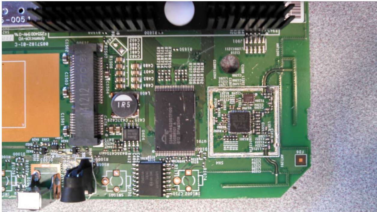
ARRIS IP815 INTERNAL RF4CE SHIELDING REMOVED
