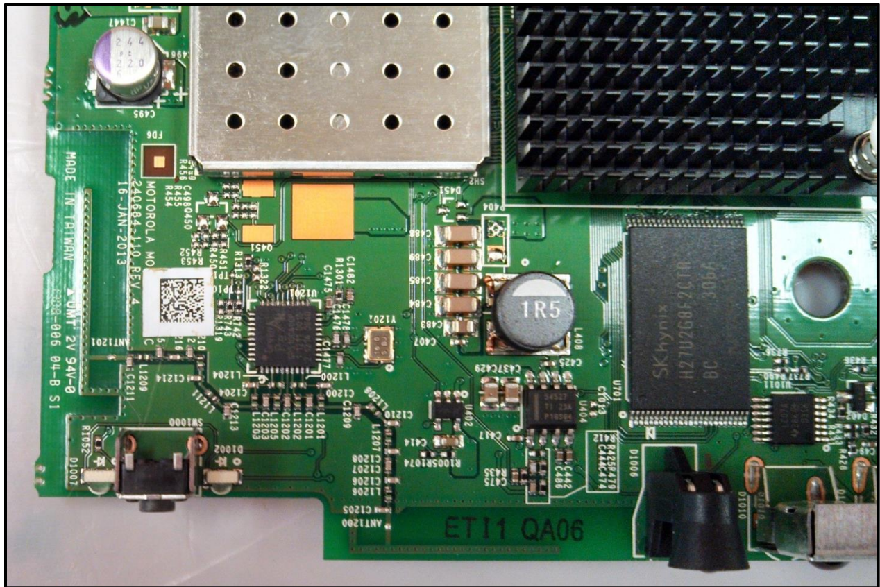
Photograph 12: Top TX
