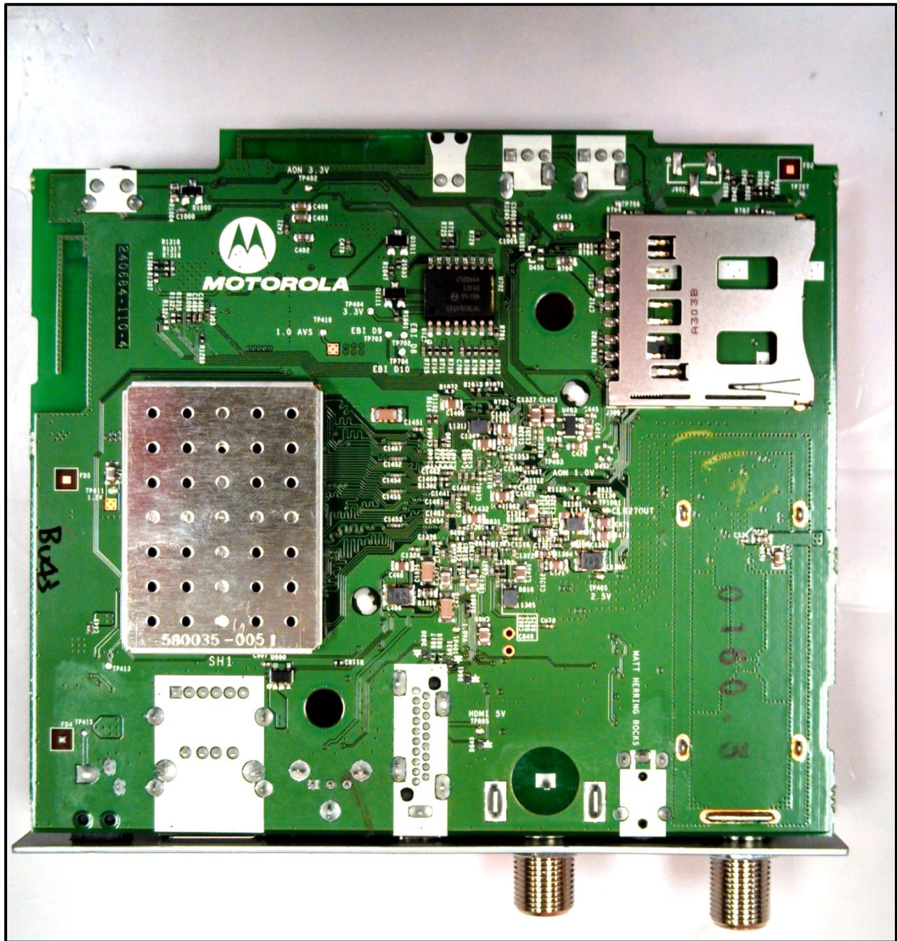
Photograph 13: Bottom PWB
